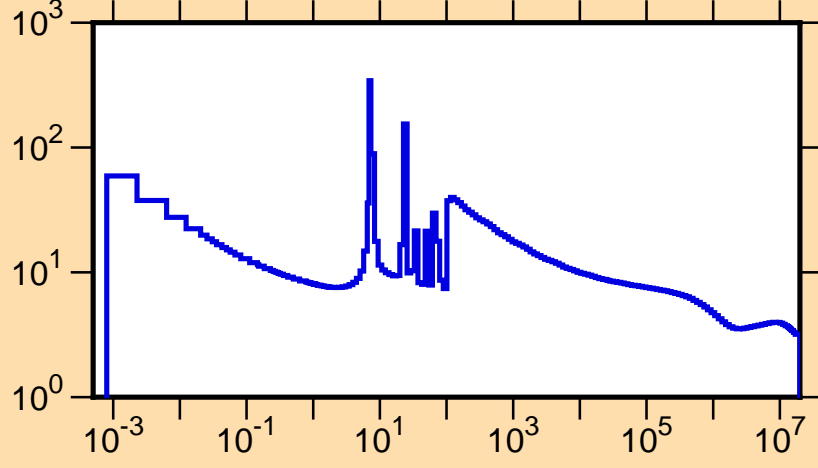
\sigma vs. E for ^{79}\text{Kr}(n,\text{tot.})
