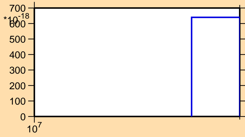
\sigma vs. E for ^{79}\text{Kr}(n,nt)
