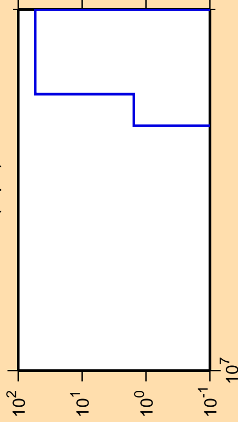
\Delta\sigma/\sigma vs. E for ^{80}\text{Kr}(n,pd)
