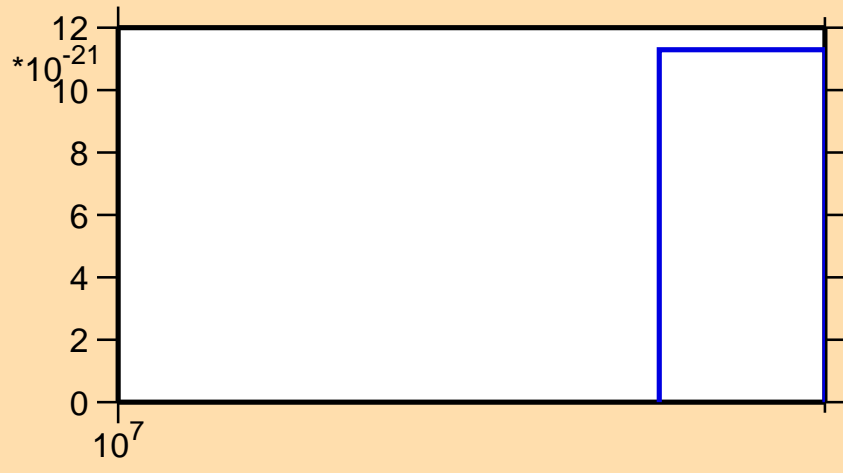
\sigma vs. E for ^{80}\text{Kr}(n,nt)
