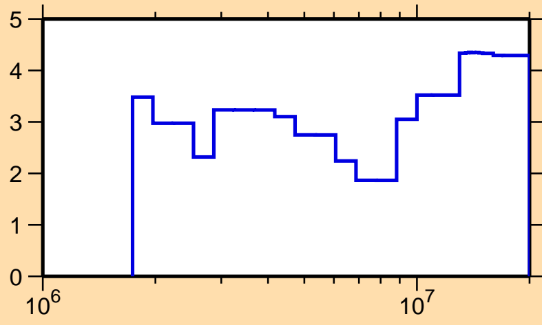
\Delta\sigma/\sigma vs. E for ^{80}\text{Kr}(n,el.)
