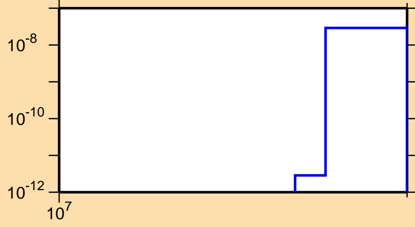
\sigma vs. E for ^{80}\text{Kr}(n,pd)
