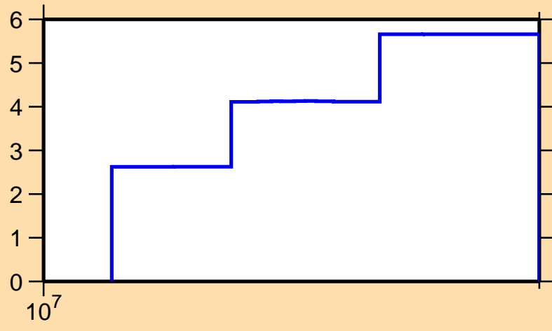
\Delta\sigma/\sigma vs. E for ^{80}\text{Kr}(n,\text{inel.})
