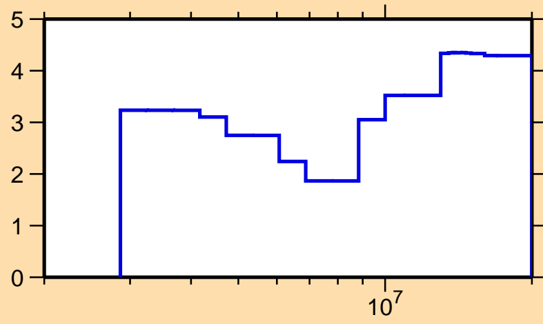
\Delta\sigma/\sigma vs. E for ^{80}\text{Kr}(n,\text{el.})
