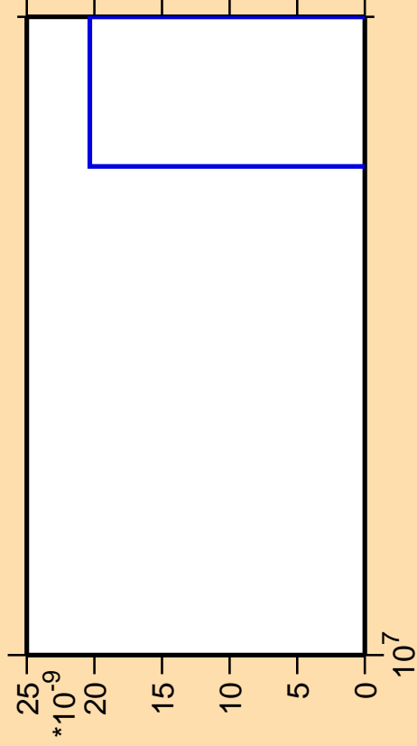
\Delta\sigma/\sigma vs. E for ^{80}\text{Kr} (mt 34)
