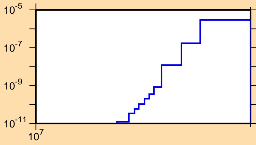
\sigma vs. E for ^{80}\text{Kr}(n,\text{He}3)
