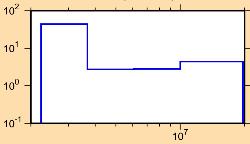
\Delta\sigma/\sigma vs. E for ^{80}\text{Kr}(n,n\text{cont.})
