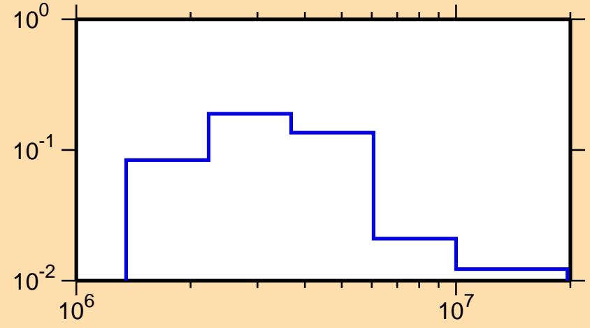
\sigma vs. E for ^{80}\text{Kr}(n,n_4)
