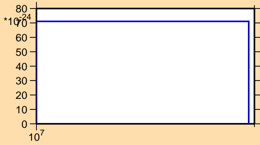
\sigma vs. E for ^{80}\text{Kr} (mt 34)
