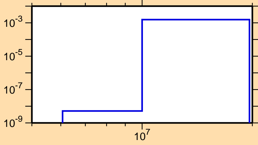
\sigma vs. E for ^{80}\text{Kr}(n,n\alpha)
