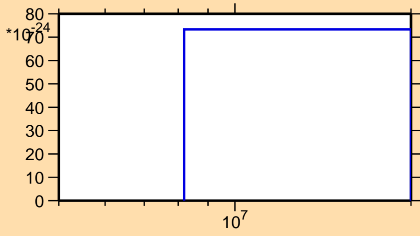
\sigma vs. E for ^{80}\text{Kr}(\text{mt } 34)
