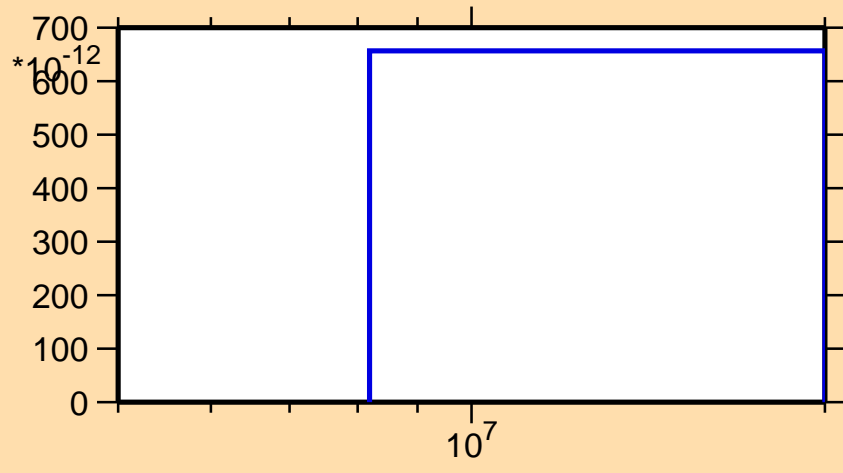
\sigma vs. E for ^{80}\text{Kr}(n,p\alpha)
