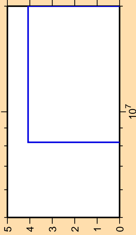
\Delta\sigma/\sigma vs. E for ^{80}\text{Kr}(n,2n)
