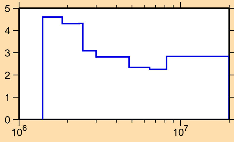
\Delta\sigma/\sigma vs. E for ^{80}\text{Kr}(n,\text{inel.})
