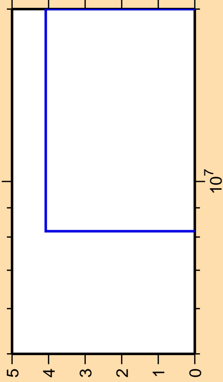
\Delta\sigma/\sigma vs. E for ^{80}\text{Kr}(n,2n)
