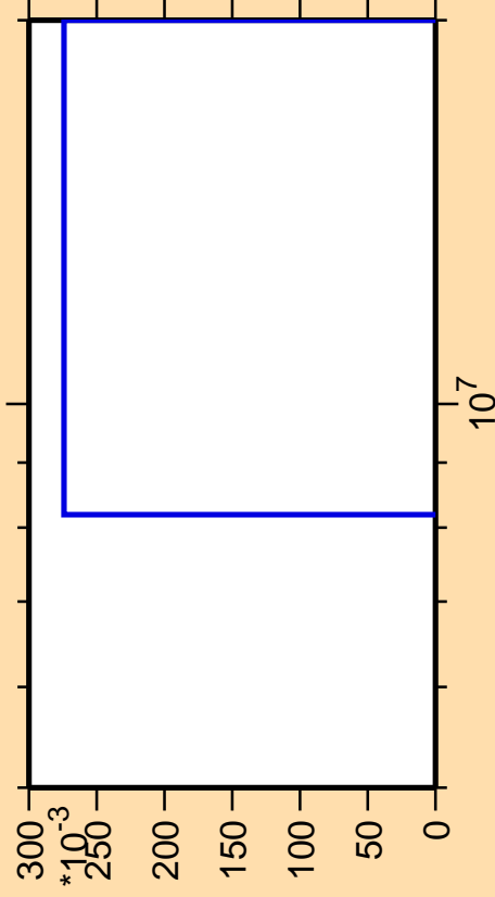
\Delta\sigma/\sigma vs. E for ^{80}\text{Kr}(n,\text{nd})
