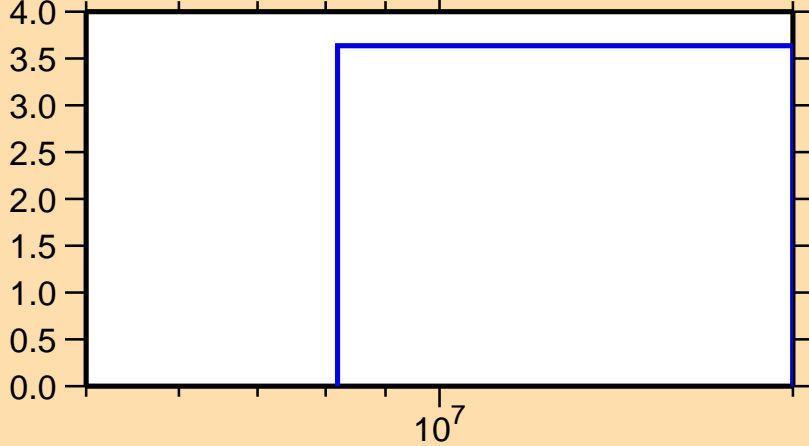
\Delta\sigma/\sigma vs. E for ^{80}\text{Kr}(n,\text{el.})
