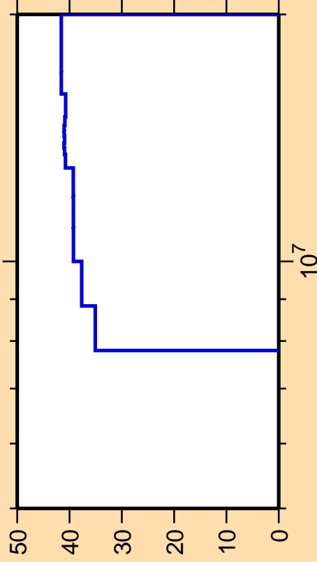
\Delta\sigma/\sigma vs. E for ^{81}\text{Kr}(n,\gamma)
