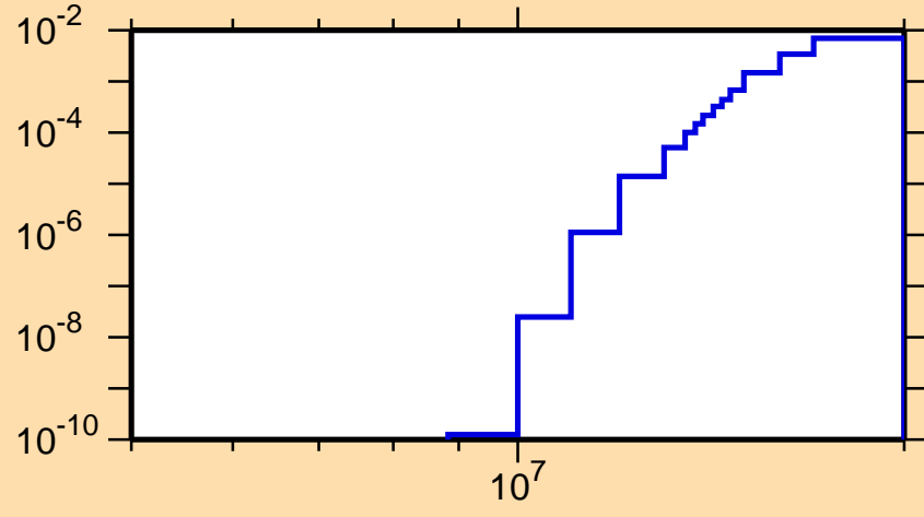
\sigma vs. E for ^{81}\text{Kr}(n,\alpha)
