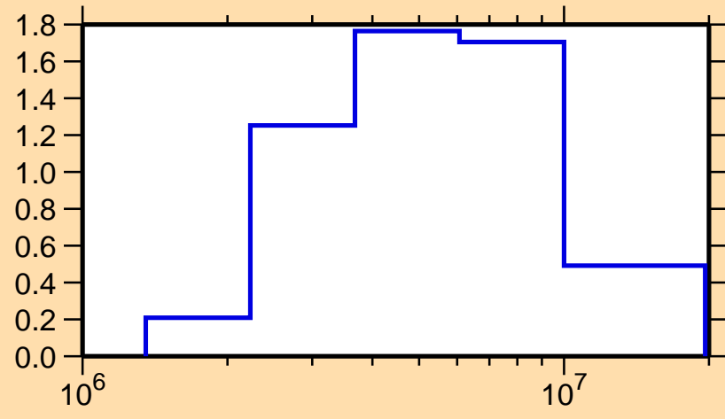
\sigma vs. E for ^{81}\text{Kr}(n,n\text{cont.})
