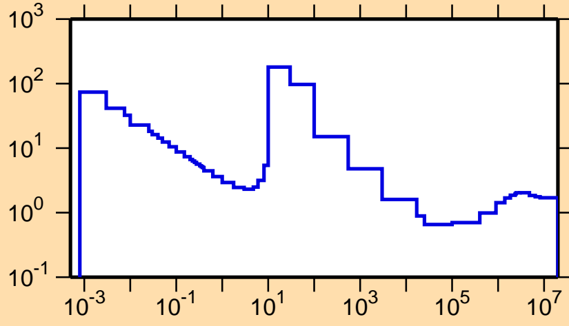
\sigma vs. E for ^{81}\text{Kr}(n,\text{nonel.})
