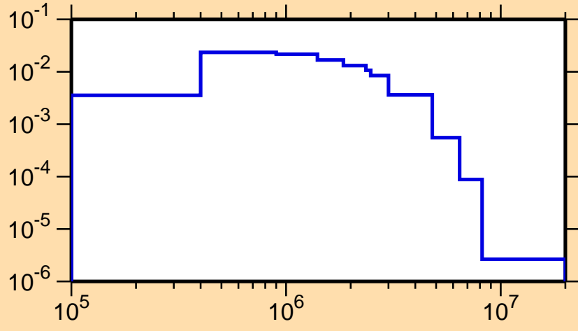
\sigma vs. E for ^{81}\text{Kr}(n,n_2)
