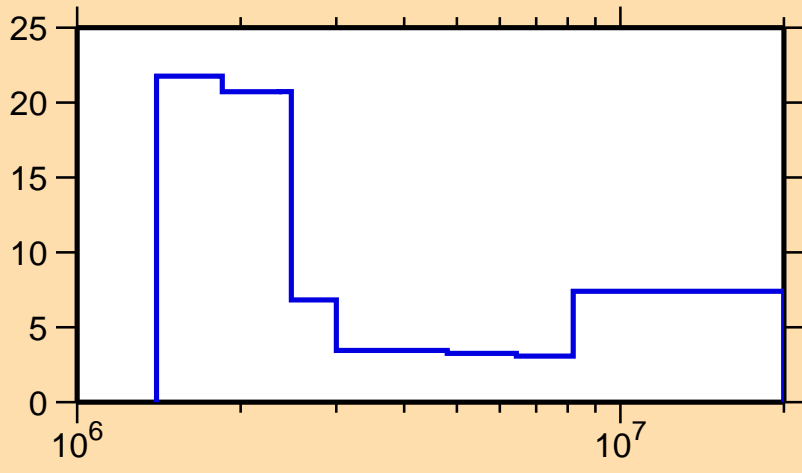
\Delta\sigma/\sigma vs. E for ^{81}\text{Kr}(n,n\text{cont.})
