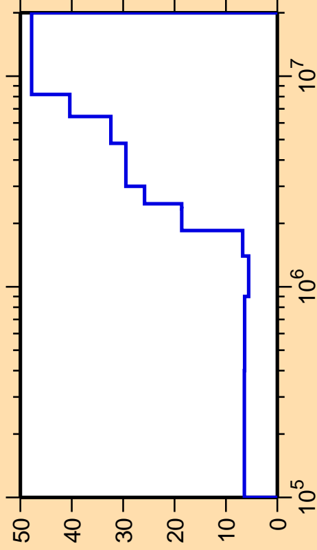
\Delta\sigma/\sigma vs. E for ^{81}\text{Kr}(n,n_2)
