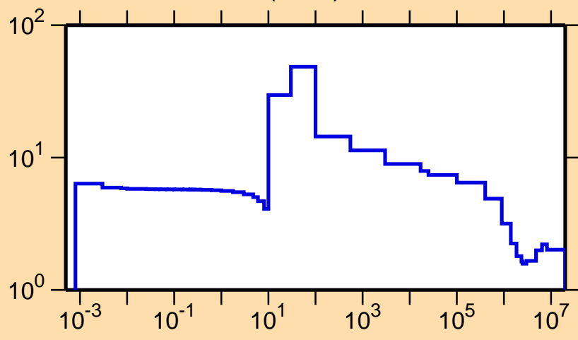
\sigma vs. E for ^{81}\text{Kr}(n,\text{el.})
