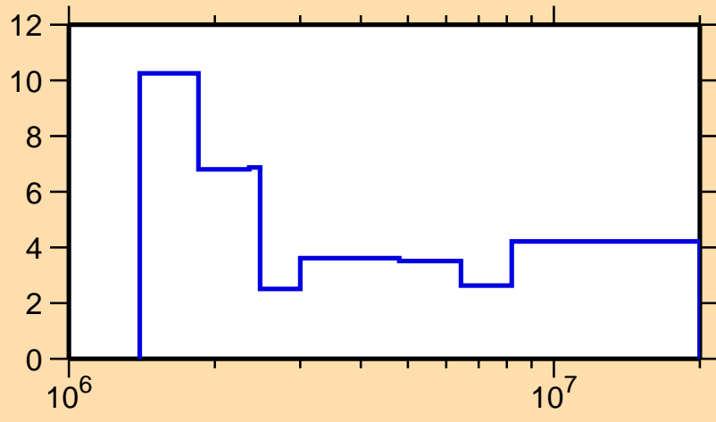
\Delta\sigma/\sigma vs. E for ^{81}\text{Kr}(n, el.)
