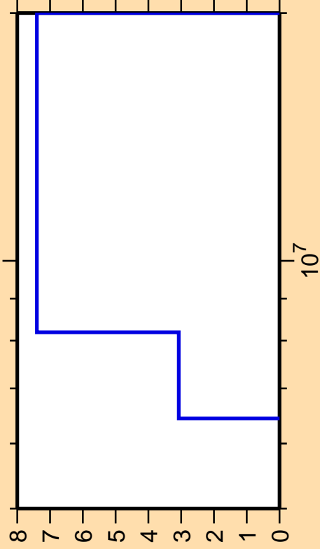
\Delta\sigma/\sigma vs. E for ^{81}\text{Kr}(n,n\text{cont.})
