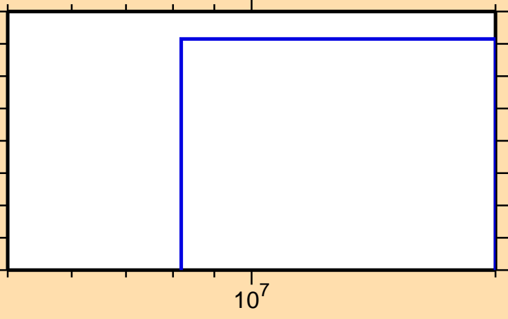
\sigma vs. E for ^{81}\text{Kr}(n,\text{pt})
