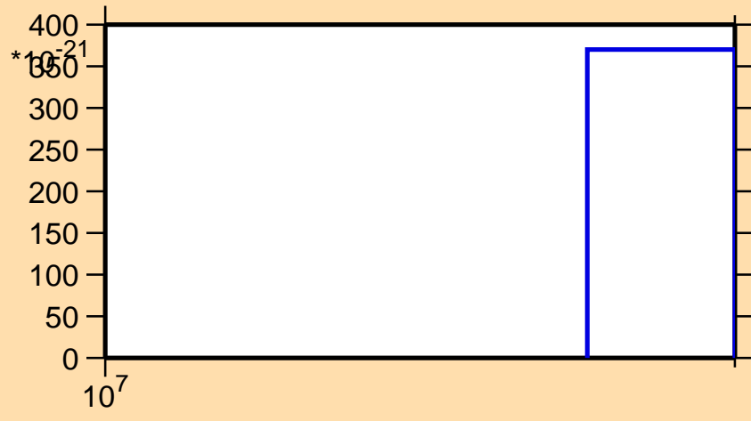
\sigma vs. E for ^{82}\text{Kr}(n,nt)
