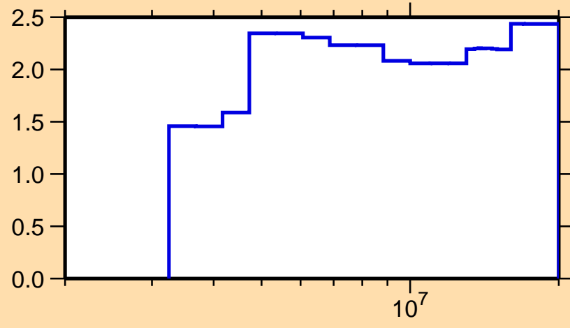
\Delta\sigma/\sigma vs. E for ^{82}\text{Kr}(n,n\text{onel.})
