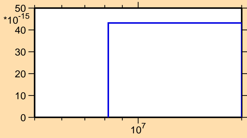
\sigma vs. E for ^{82}\text{Kr}(n,nd)
