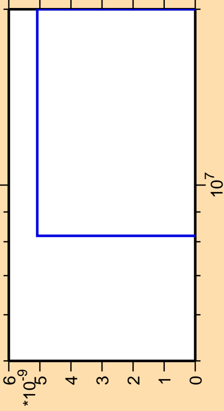
\Delta\sigma/\sigma vs. E for ^{82}\text{Kr}(n,nt)
