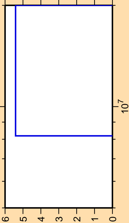
\Delta\sigma/\sigma vs. E for ^{82}\text{Kr}(n,2n)
