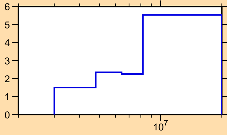
\Delta\sigma/\sigma vs. E for ^{82}\text{Kr}(n,inel.)
