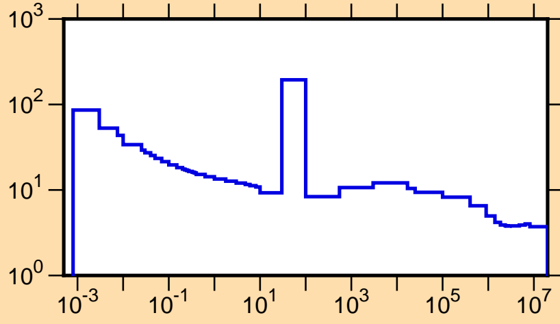
\sigma vs. E for ^{82}\text{Kr}(n,\text{tot.})
