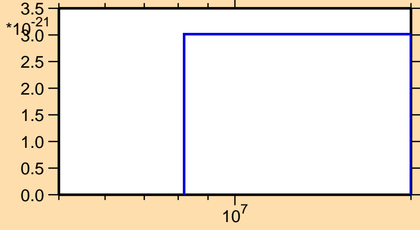
\sigma vs. E for ^{82}\text{Kr}(n,nt)
