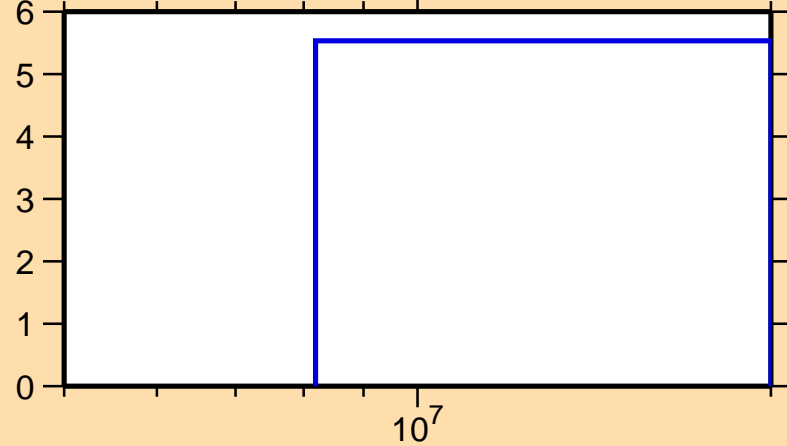
\Delta\sigma/\sigma vs. E for ^{82}\text{Kr}(n,\text{inel.})
