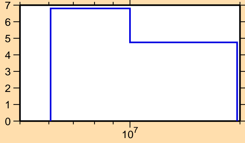
\Delta\sigma/\sigma vs. E for ^{83}\text{Kr}(n,2n)
