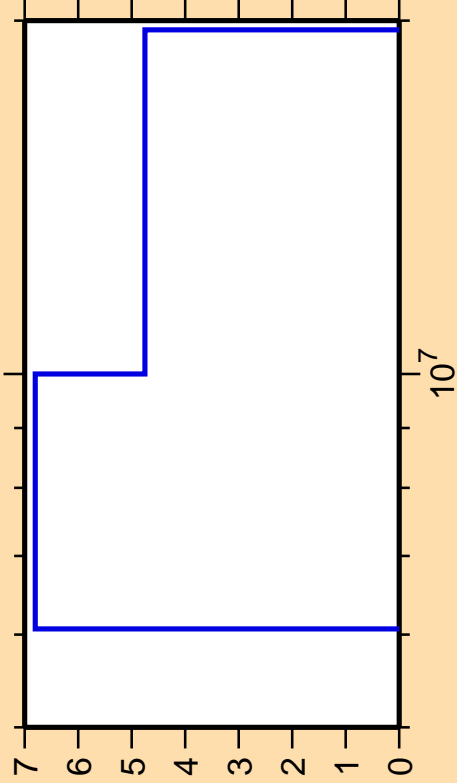
\Delta\sigma/\sigma vs. E for ^{83}\text{Kr}(n,2n)
