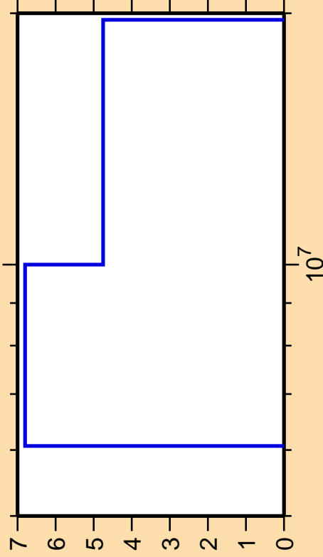
\Delta\sigma/\sigma vs. E for ^{83}\text{Kr}(n,2n)
