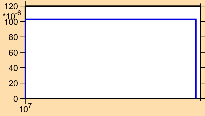
\sigma vs. E for ^{83}\text{Kr}(n,t)
