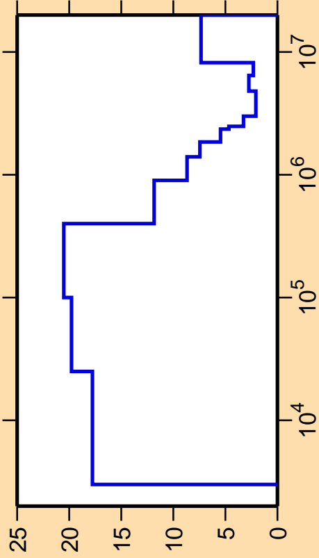
\Delta\sigma/\sigma vs. E for ^{83}\text{Kr}(n,\text{inel.})
