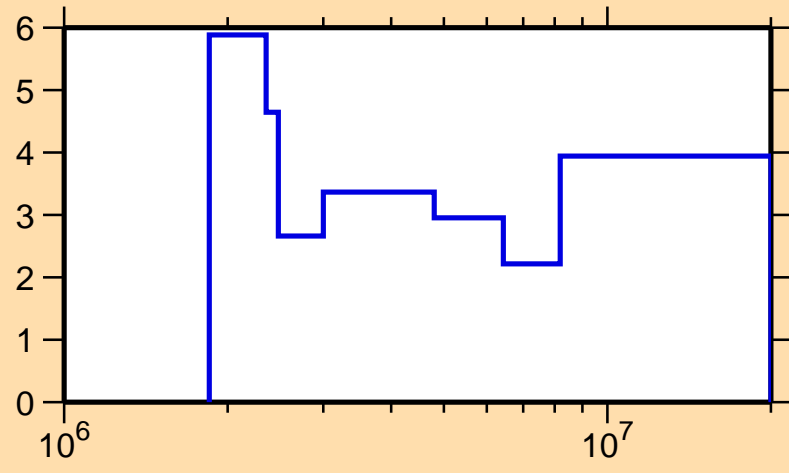
\Delta\sigma/\sigma vs. E for ^{83}\text{Kr}(n, el.)
