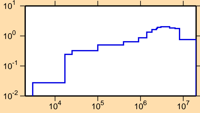
\sigma vs. E for ^{83}\text{Kr}(n,\text{inel.})
