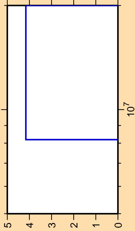
\Delta\sigma/\sigma vs. E for ^{83}\text{Kr}(n,2np)
