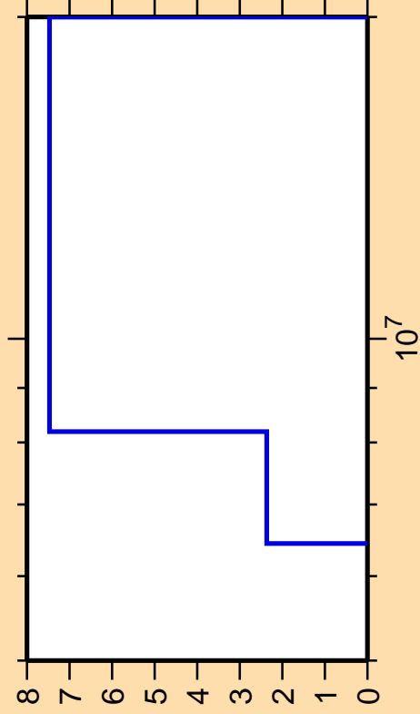
\Delta\sigma/\sigma vs. E for ^{83}\text{Kr}(n,n\text{cont.})
