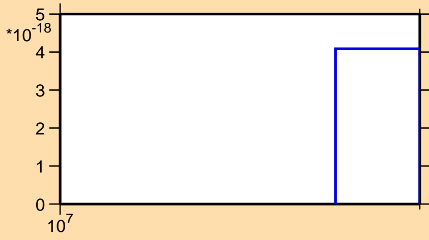
\sigma vs. E for ^{84}\text{Kr}(n,nt)
