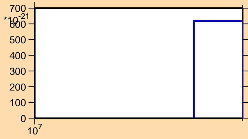
\sigma vs. E for ^{84}\text{Kr}(n,2n\alpha)
