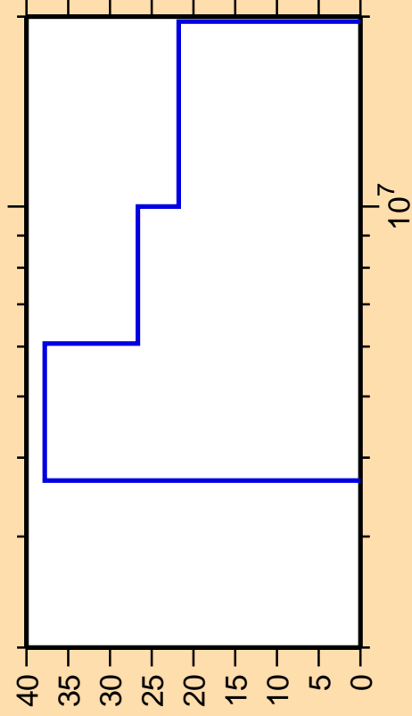
\Delta\sigma/\sigma vs. E for ^{84}\text{Kr}(n,p)
