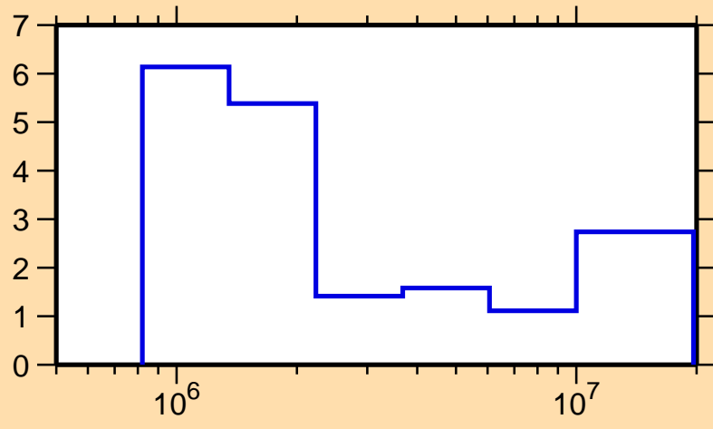
\Delta\sigma/\sigma vs. E for ^{84}\text{Kr}(n,\text{tot.})
