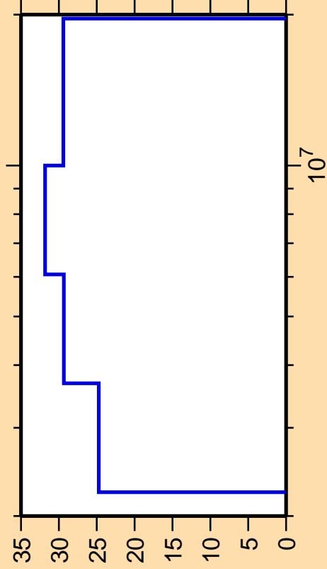
\Delta\sigma/\sigma vs. E for ^{84}\text{Kr}(n,\gamma)
