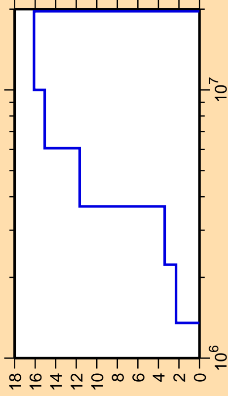
\Delta\sigma/\sigma vs. E for ^{84}\text{Kr}(n,n_2)
