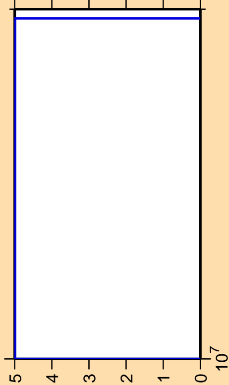
\Delta\sigma/\sigma vs. E for ^{84}\text{Kr}(n,2n)
