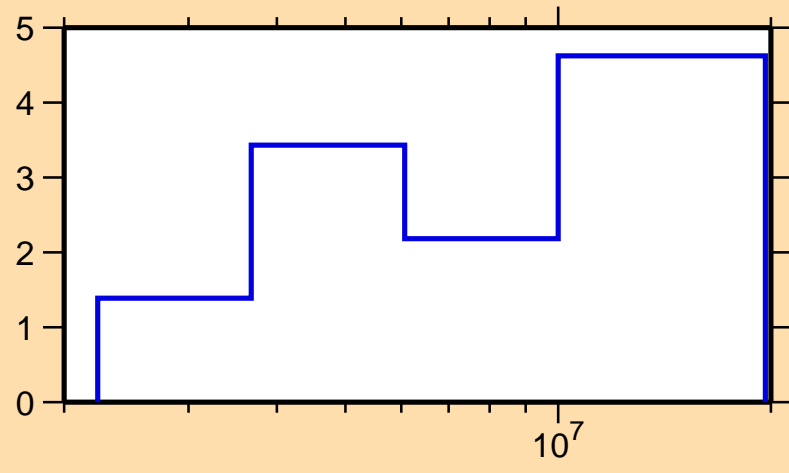
\Delta\sigma/\sigma vs. E for ^{84}\text{Kr}(n,el.)
