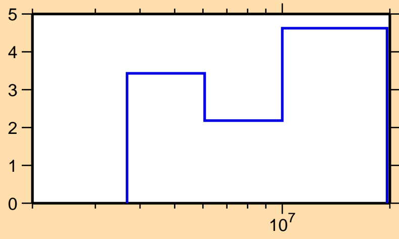
\Delta\sigma/\sigma vs. E for ^{84}\text{Kr}(n,\text{el.})
