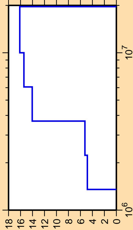
\Delta\sigma/\sigma vs. E for ^{84}\text{Kr}(n,n_4)
