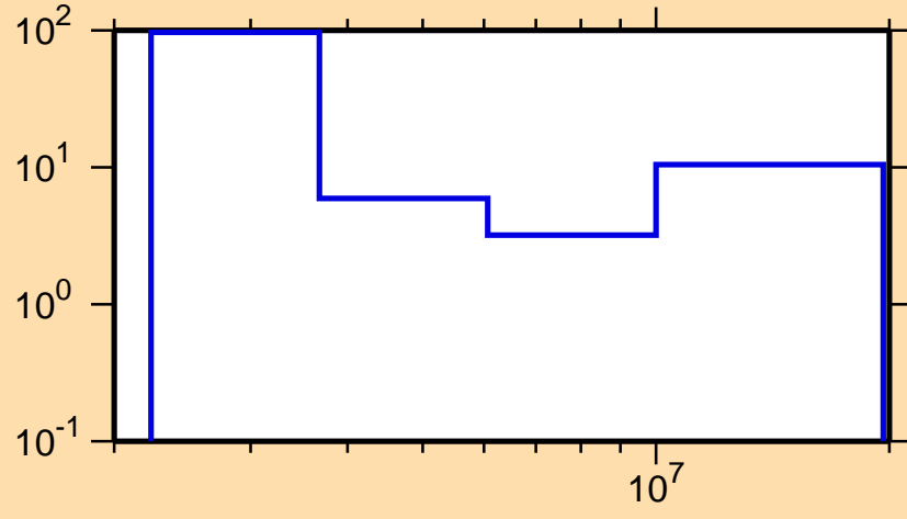
\Delta\sigma/\sigma vs. E for ^{84}\text{Kr}(n,n\text{cont.})
