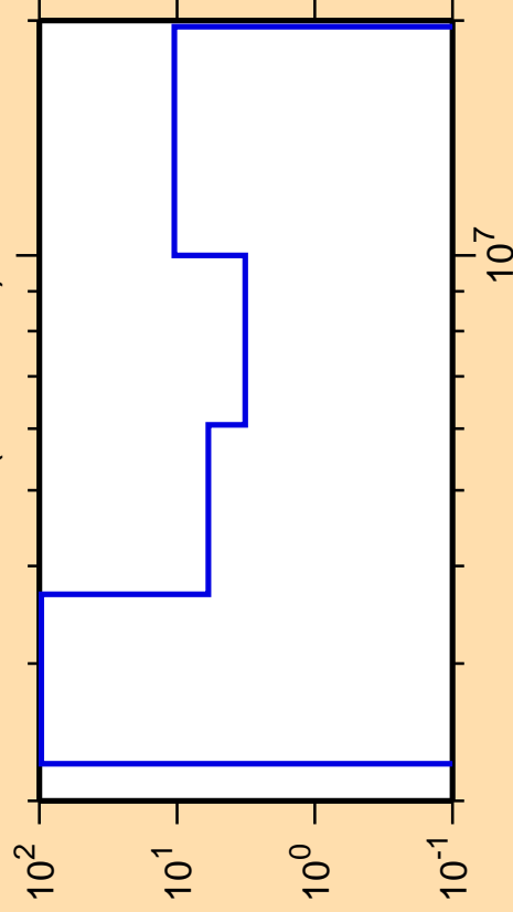
\Delta\sigma/\sigma vs. E for ^{84}\text{Kr}(n,ncont.)
