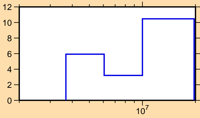
\Delta\sigma/\sigma vs. E for ^{84}\text{Kr}(n,ncont.)
