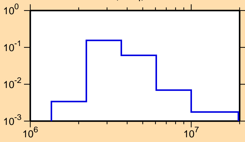
\sigma vs. E for ^{84}\text{Kr}(n,n_4)
