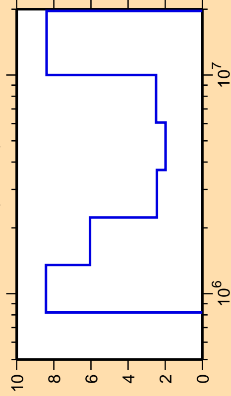
\Delta\sigma/\sigma vs. E for ^{84}\text{Kr}(n,\text{inel.})
