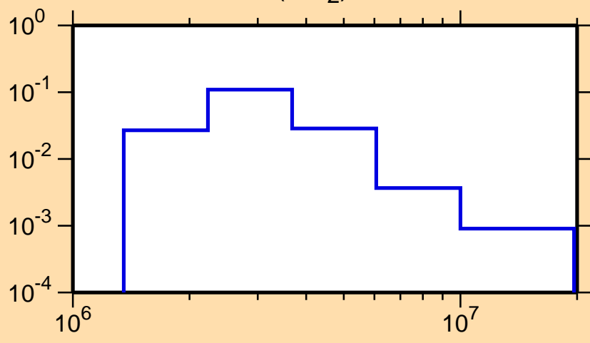
\sigma vs. E for ^{84}\text{Kr}(n,n_2)
