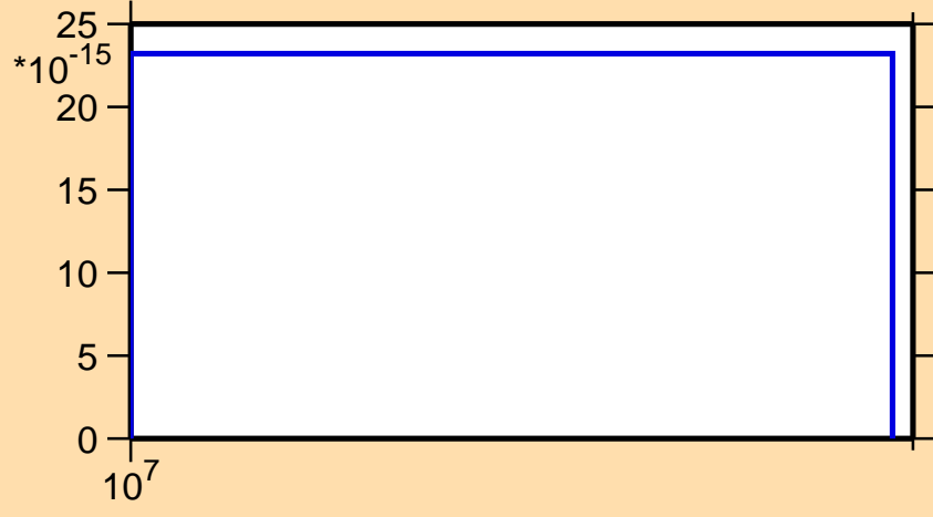
\sigma vs. E for ^{84}\text{Kr}(n,\text{nd})
