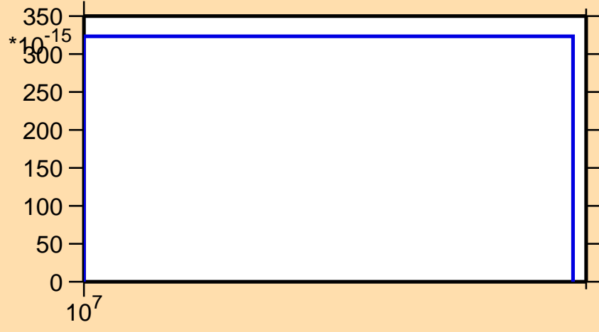
\sigma vs. E for ^{84}\text{Kr}(n,\text{He}3)
