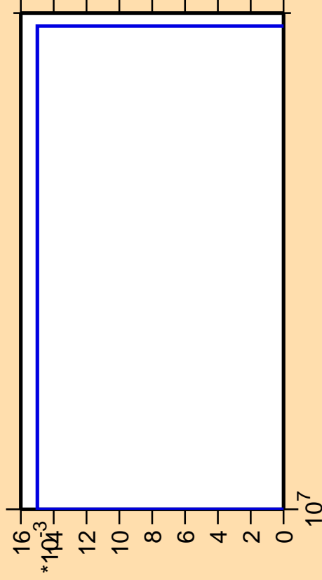
\Delta\sigma/\sigma vs. E for ^{84}\text{Kr}(n,\text{nd})
