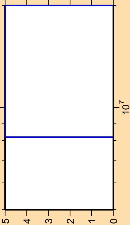
\Delta\sigma/\sigma vs. E for ^{84}\text{Kr}(n,2n)
