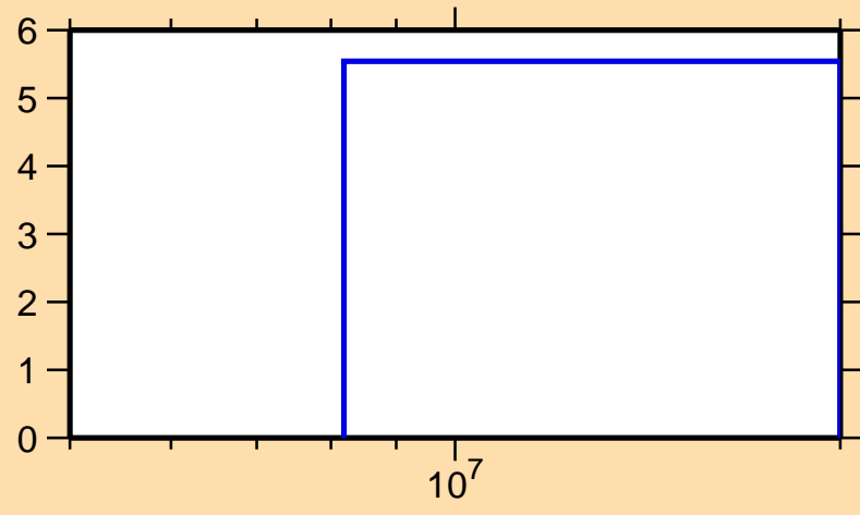
\Delta\sigma/\sigma vs. E for ^{84}\text{Kr}(n,\text{inel.})
