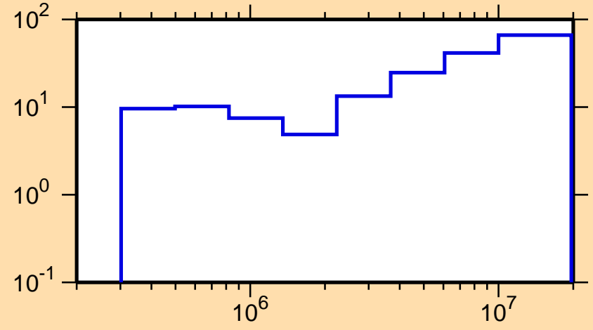
\Delta\sigma/\sigma vs. E for ^{85}\text{Kr}(n,n_1)
