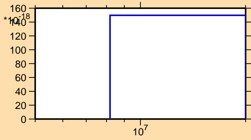
\sigma vs. E for ^{85}\text{Kr}(n,nt)
