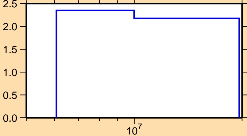
\Delta\sigma/\sigma vs. E for ^{85}\text{Kr}(n,\text{nonel.})
