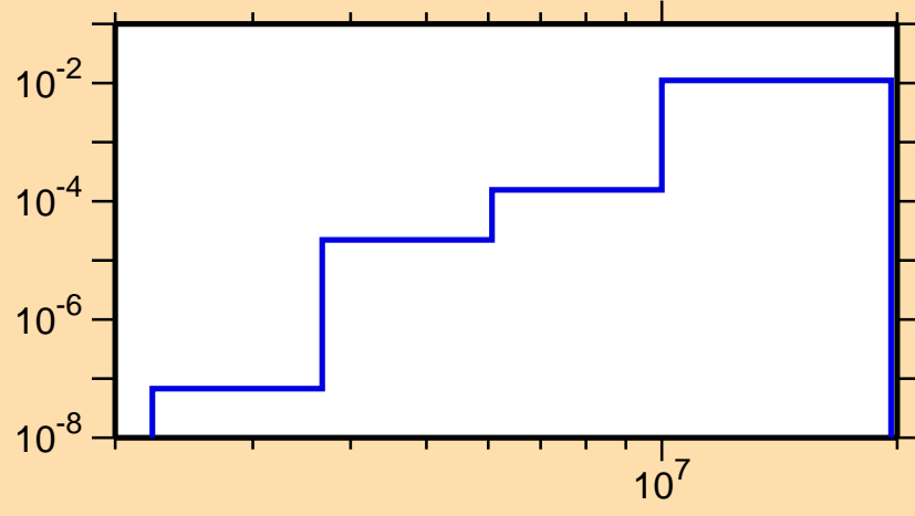
\sigma vs. E for ^{85}\text{Kr}(n,p)
