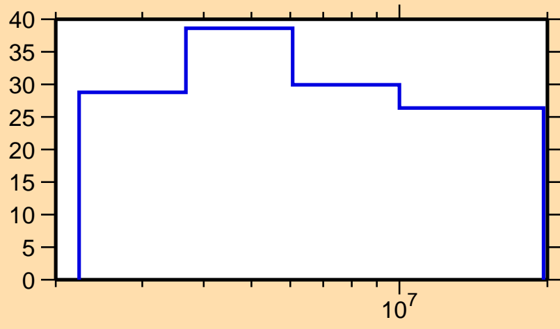
\Delta\sigma/\sigma vs. E for ^{85}\text{Kr}(n,p)
