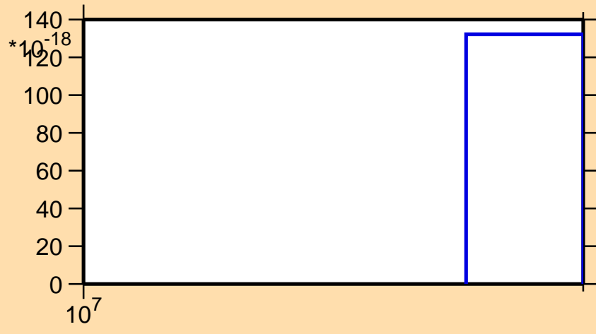
\sigma vs. E for ^{86}\text{Kr}(n,nt)
