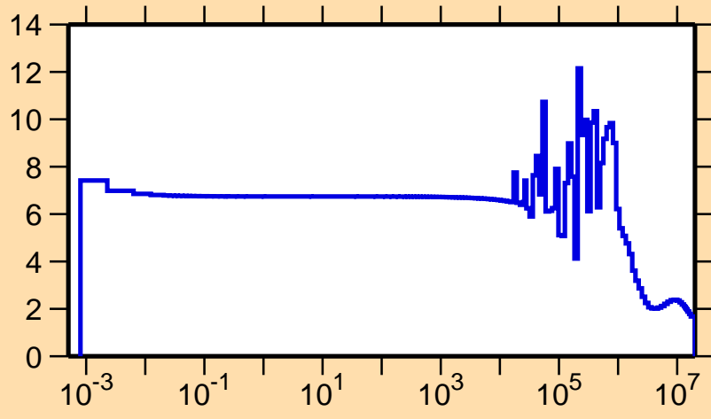
\sigma vs. E for ^{86}\text{Kr}(n,\text{el.})
