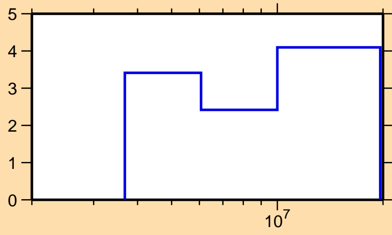
\Delta\sigma/\sigma vs. E for ^{86}\text{Kr}(n,el.)
