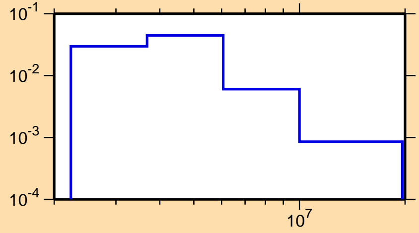
\sigma vs. E for ^{86}\text{Kr}(n,n_4)
