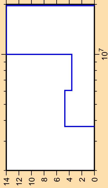
\Delta\sigma/\sigma vs. E for ^{86}\text{Kr}(n,ncont.)
