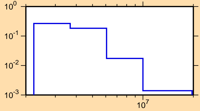
\sigma vs. E for ^{86}\text{Kr}(n,n_3)
