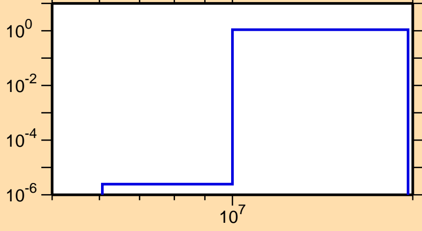
\sigma vs. E for ^{86}\text{Kr}(n,2n)
