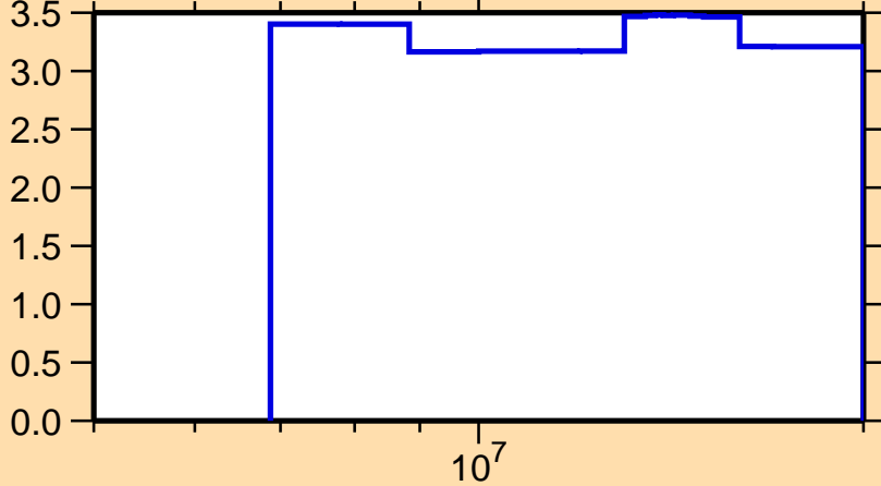
\Delta\sigma/\sigma vs. E for ^{88}\text{Kr}(n,\text{nonel.})
