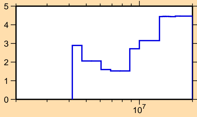
\Delta\sigma/\sigma vs. E for ^{88}\text{Kr}(n,\text{tot.})
