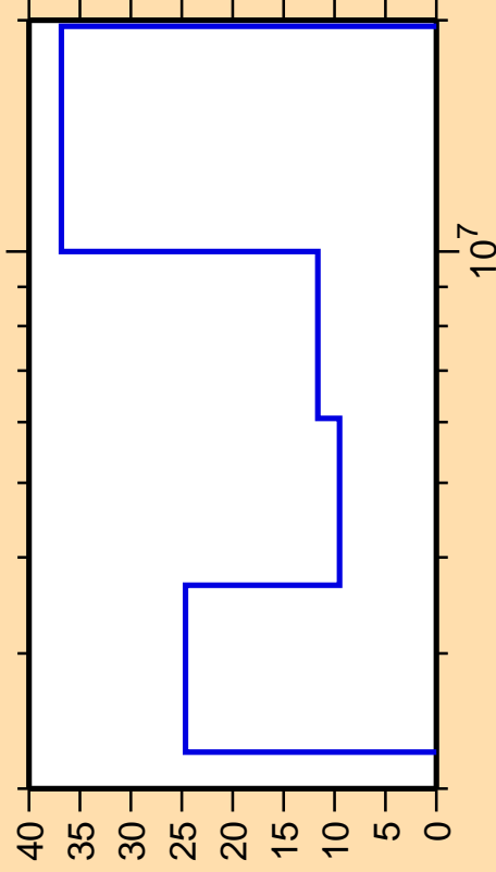
\Delta\sigma/\sigma vs. E for ^{88}\text{Kr}(n,ncont.)
