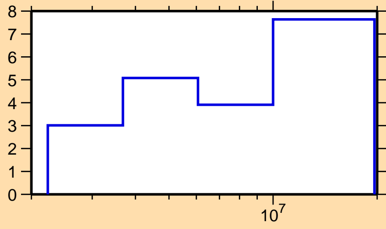
\Delta\sigma/\sigma vs. E for ^{88}\text{Kr}(n,el.)
