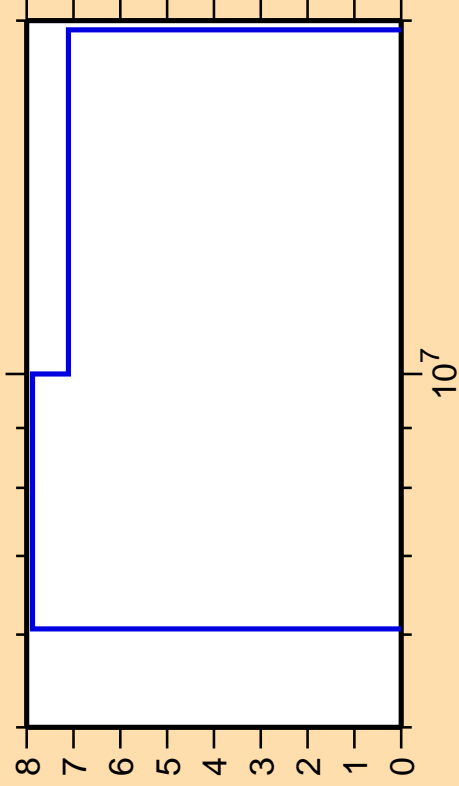
\Delta\sigma/\sigma vs. E for ^{88}\text{Kr}(n,2n)
