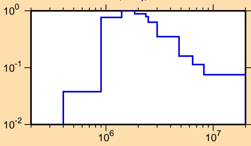
\sigma vs. E for ^{88}\text{Kr}(n,n_1)
