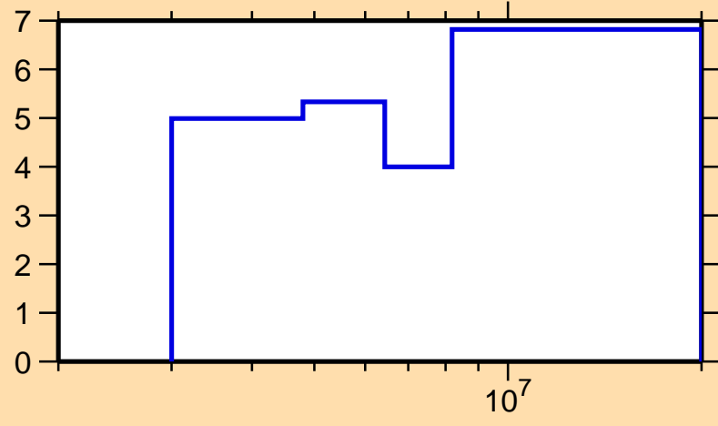
\Delta\sigma/\sigma vs. E for ^{88}\text{Kr}(n,\text{el.})
