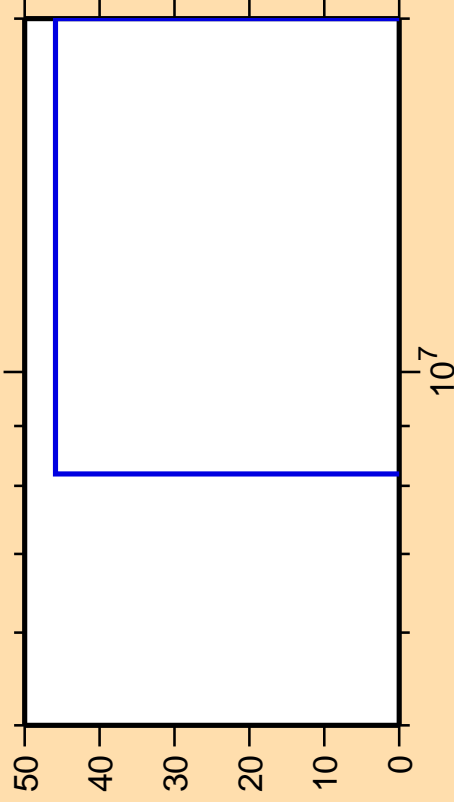
\Delta\sigma/\sigma vs. E for ^{88}\text{Kr}(n,p)
