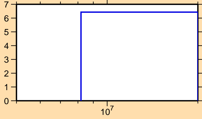
\Delta\sigma/\sigma vs. E for ^{88}\text{Kr}(n,2n)
