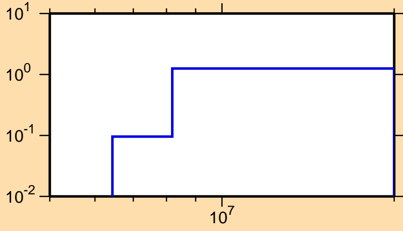
\sigma vs. E for ^{88}\text{Kr}(n,2n)
