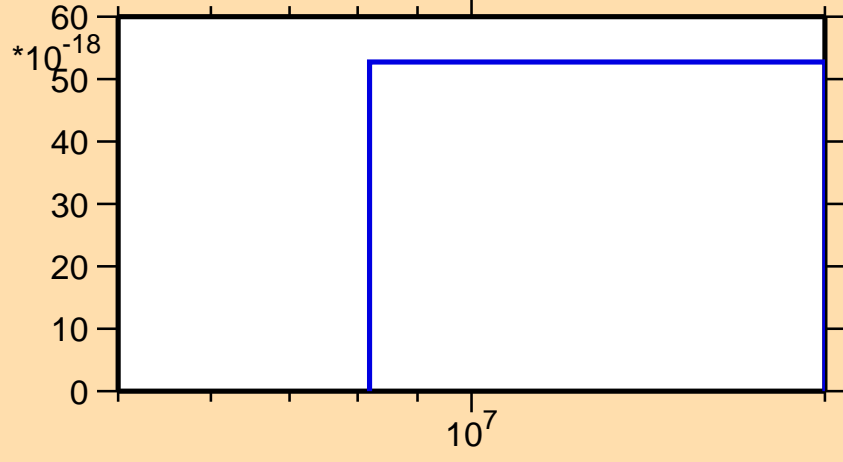
\sigma vs. E for ^{88}\text{Kr}(n,2np)
