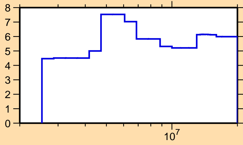
\Delta\sigma/\sigma vs. E for ^{89}\text{Kr}(n,\text{nonel.})
