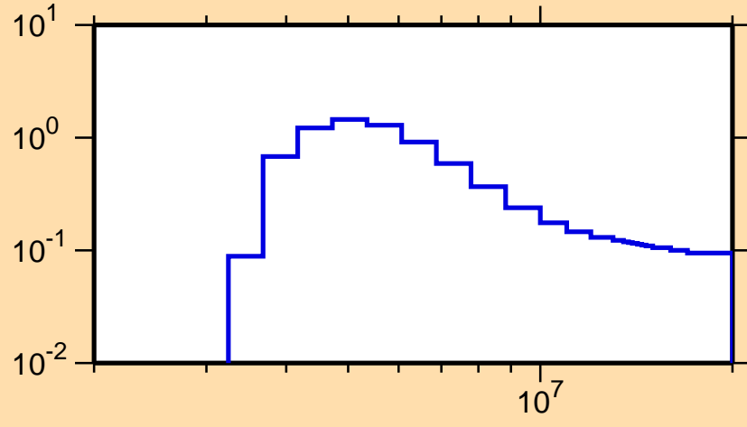
\sigma vs. E for ^{89}\text{Kr}(n,n\text{cont.})
