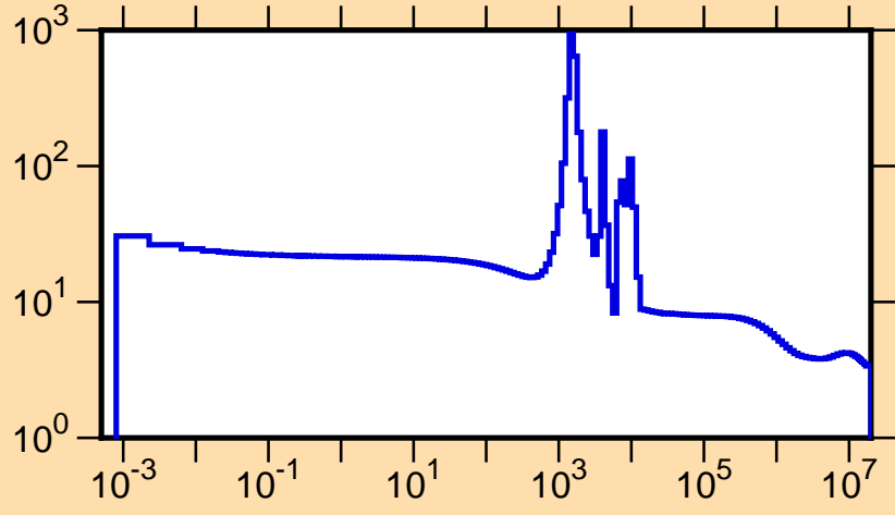
\sigma vs. E for ^{89}\text{Kr}(n,\text{tot.})
