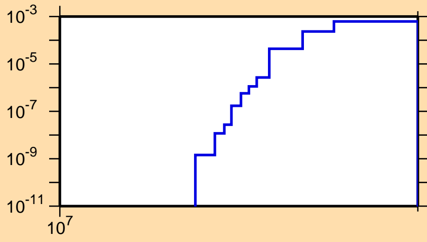
\sigma vs. E for ^{89}\text{Kr}(n,d)
