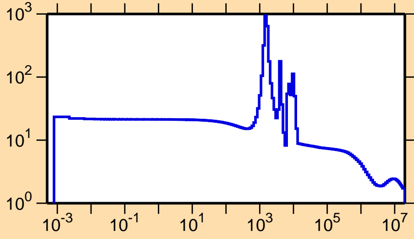
\sigma vs. E for ^{89}\text{Kr}(n,\text{el.})
