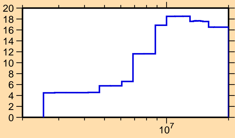
\Delta\sigma/\sigma vs. E for ^{89}\text{Kr}(n,\text{inel.})
