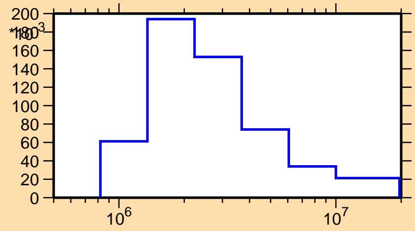
\sigma vs. E for ^{89}\text{Kr}(n,n_4)
