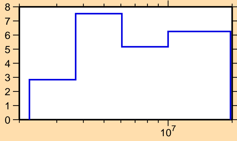
\Delta\sigma/\sigma vs. E for ^{89}\text{Kr}(n,\text{el.})
