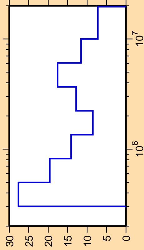
\Delta\sigma/\sigma vs. E for ^{89}\text{Kr}(n,n_2)
