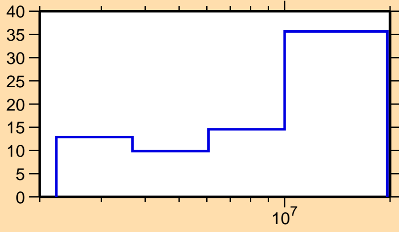
\Delta\sigma/\sigma vs. E for ^{89}\text{Kr}(n,n\text{cont.})
