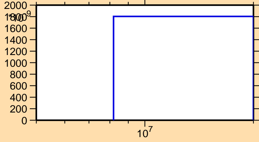
\sigma vs. E for ^{89}\text{Kr}(n,np)
