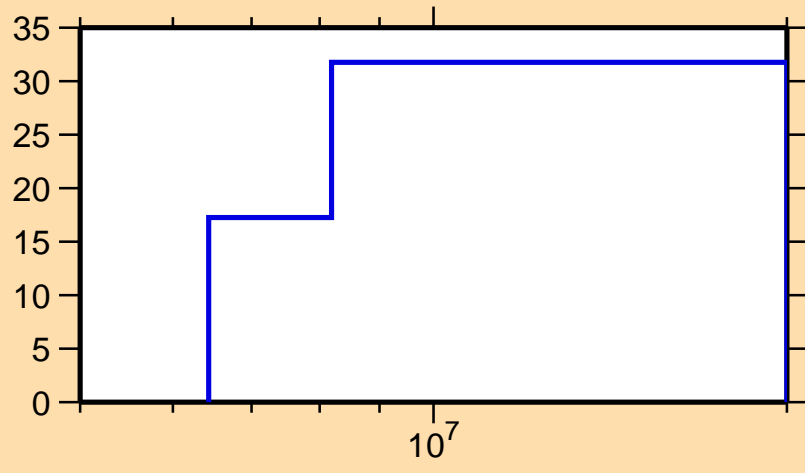
\Delta\sigma/\sigma vs. E for ^{89}\text{Kr}(n,ncont.)
