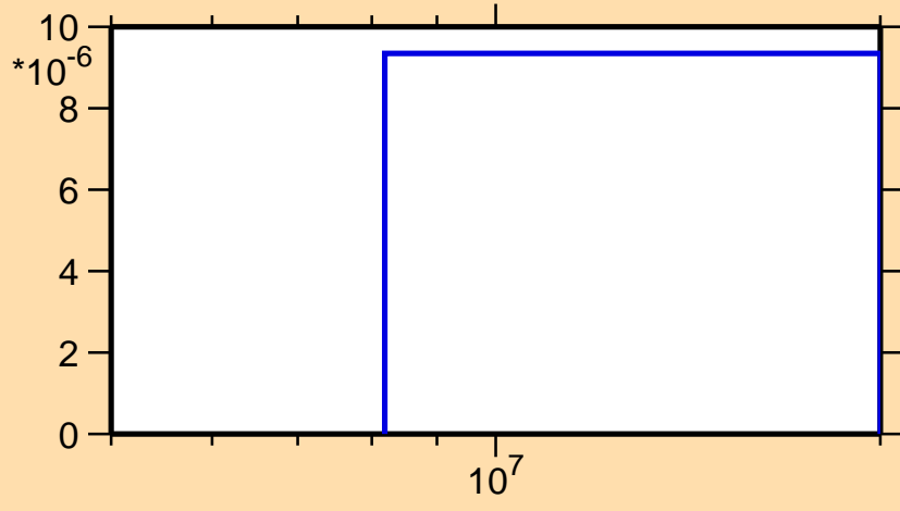
\sigma vs. E for ^{89}\text{Kr}(n,\alpha)
