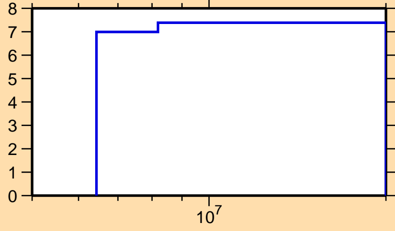
\Delta\sigma/\sigma vs. E for ^{89}\text{Kr}(n,2n)
