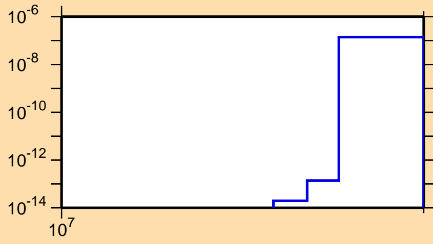
\sigma vs. E for ^{91}\text{Kr}(n,nt)
