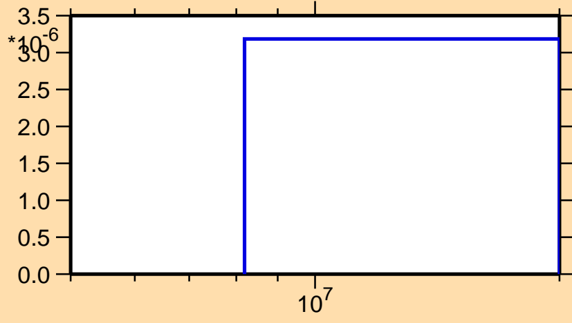
\sigma vs. E for ^{91}\text{Kr}(n,n\alpha)
