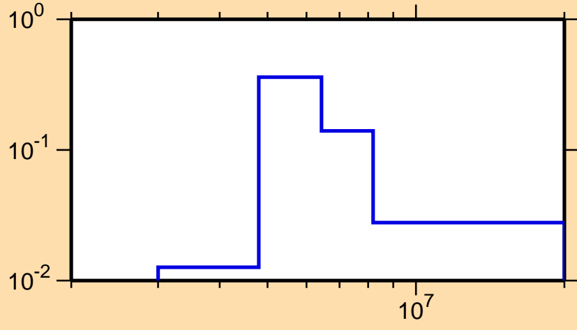
\sigma vs. E for ^{91}\text{Kr}(n,n\text{cont.})
