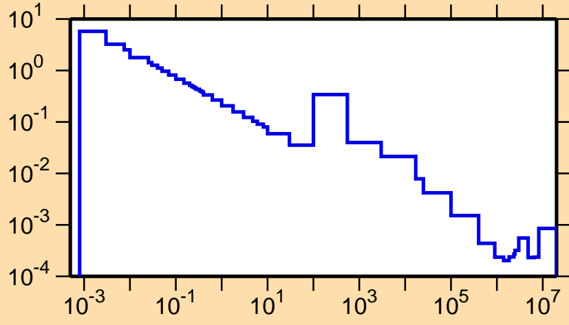
\sigma vs. E for ^{91}\text{Kr}(n,\gamma)
