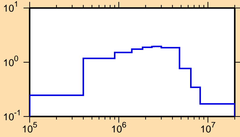
\sigma vs. E for ^{91}\text{Kr}(n,\text{inel.})
