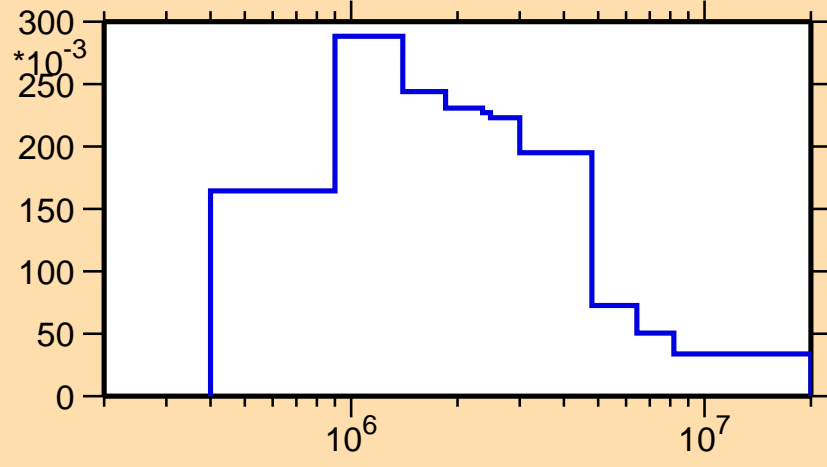
\sigma vs. E for ^{91}\text{Kr}(n,n_3)
