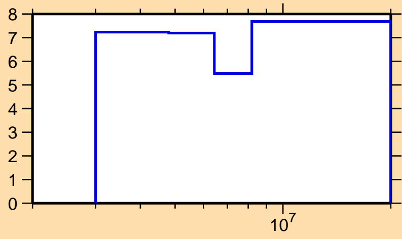
\Delta\sigma/\sigma vs. E for ^{91}\text{Kr}(n,2n)
