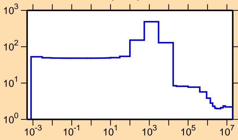
\sigma vs. E for ^{91}\text{Kr}(n,\text{el.})
