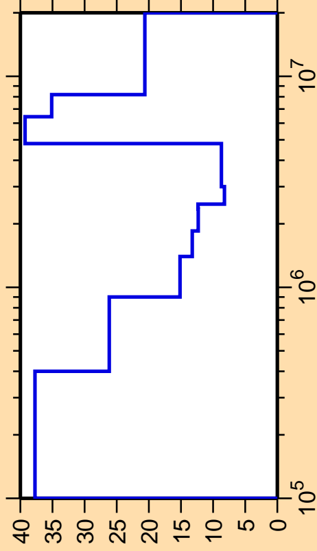
\Delta\sigma/\sigma vs. E for ^{91}\text{Kr}(n,n_2)
