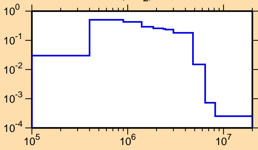
\sigma vs. E for ^{91}\text{Kr}(n,n_2)
