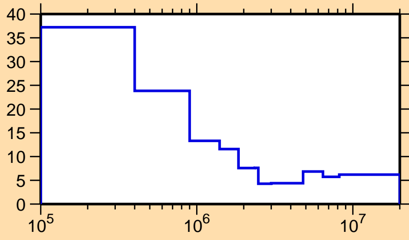
\Delta\sigma/\sigma vs. E for ^{91}\text{Kr}(n,\text{nonel.})
