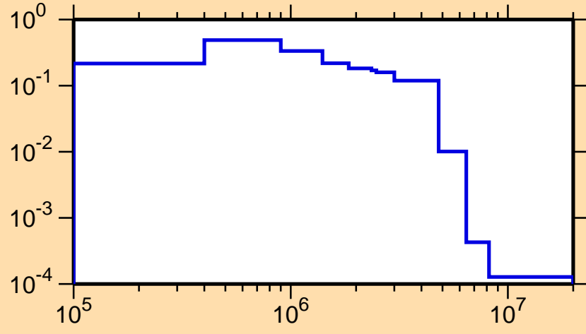
\sigma vs. E for ^{91}\text{Kr}(n,n_1)
