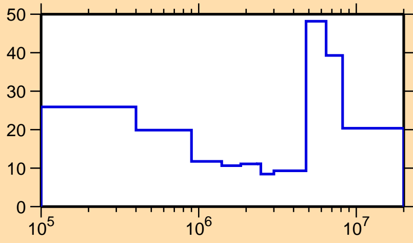
\Delta\sigma/\sigma vs. E for ^{91}\text{Kr}(n,n_1)
