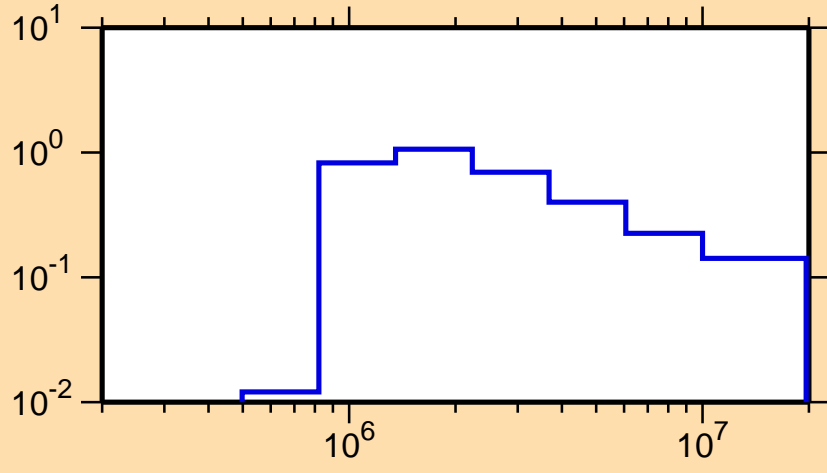
\sigma vs. E for ^{92}\text{Kr}(n,n_1)
