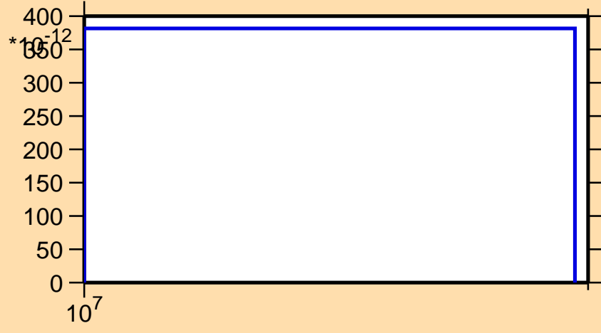
\sigma vs. E for ^{92}\text{Kr}(n,nt)
