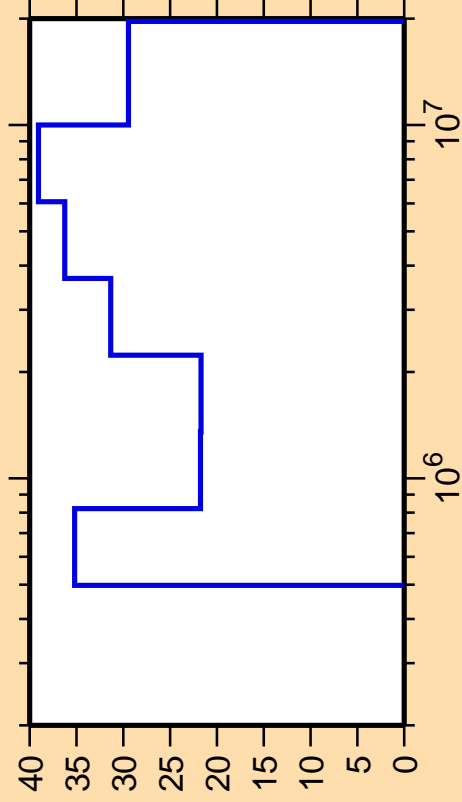
\Delta\sigma/\sigma vs. E for ^{92}\text{Kr}(n,n_1)
