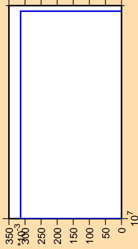
\Delta\sigma/\sigma vs. E for ^{92}\text{Kr}(n,\text{nd})
