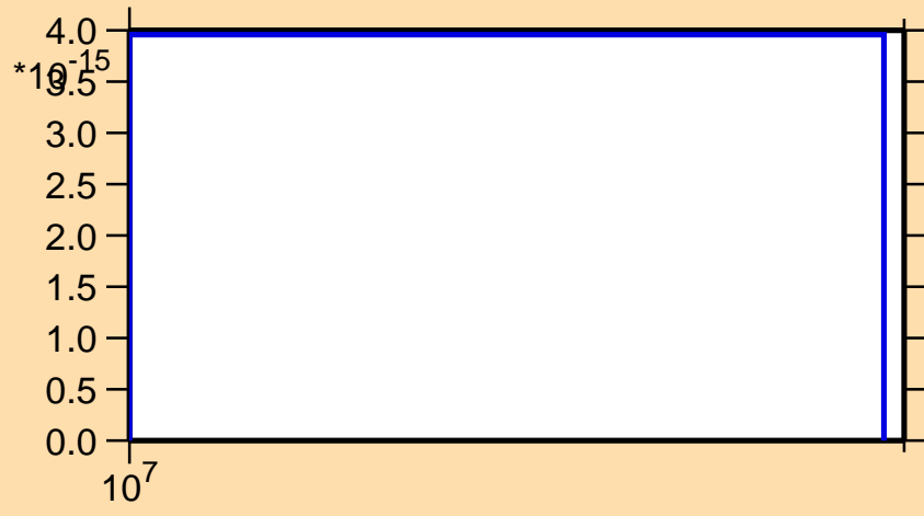
\sigma vs. E for ^{92}\text{Kr}(n,\text{nd})
