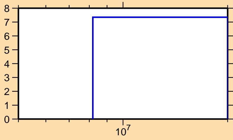
\Delta\sigma/\sigma vs. E for ^{92}\text{Kr}(n,\text{el.})
