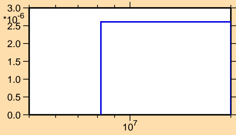
\sigma vs. E for ^{92}\text{Kr}(n,\alpha)
