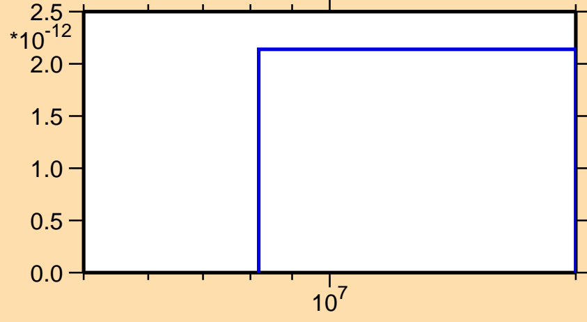
\sigma vs. E for ^{92}\text{Kr}(n,2n\alpha)
