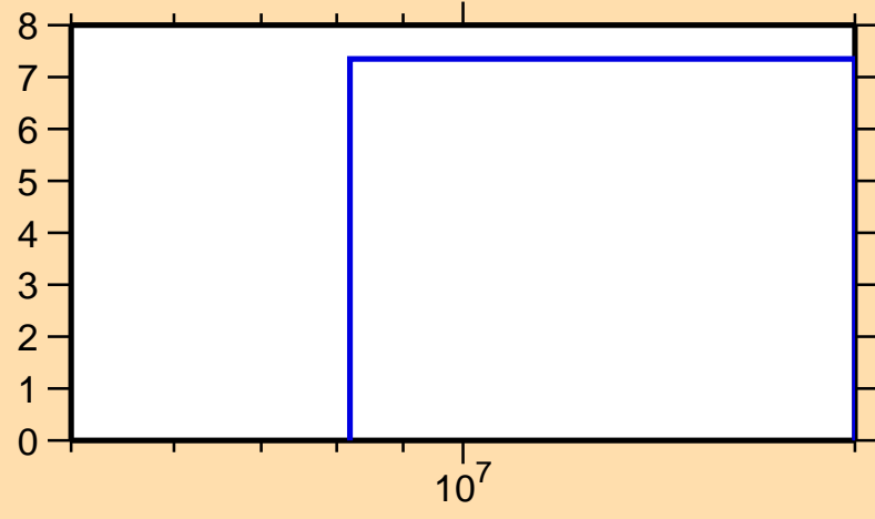
\Delta\sigma/\sigma vs. E for ^{92}\text{Kr}(n,el.)
