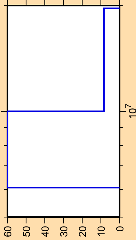
\Delta\sigma/\sigma vs. E for ^{93}\text{Kr}(n,3n)
