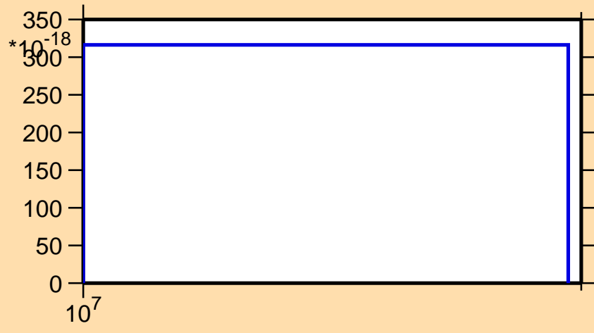
\sigma vs. E for ^{93}\text{Kr}(n,2np)
