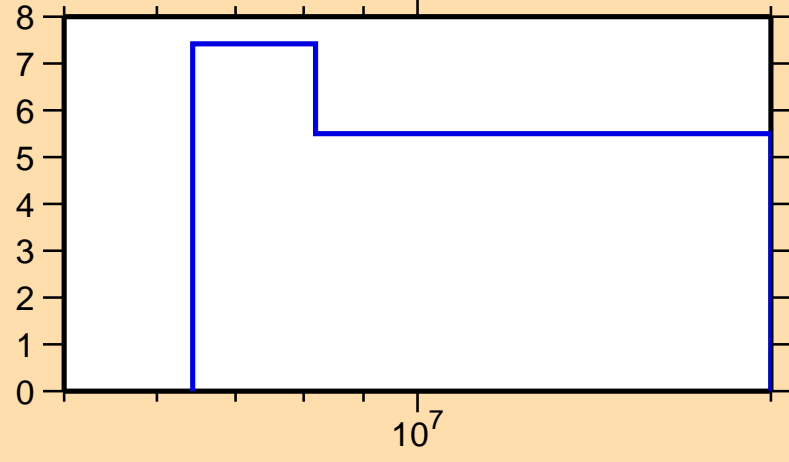
\Delta\sigma/\sigma vs. E for ^{93}\text{Kr}(n,\text{nonel.})
