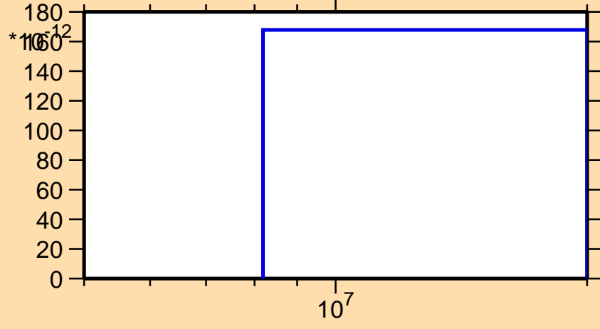
\sigma vs. E for ^{93}\text{Kr}(n,nd)
