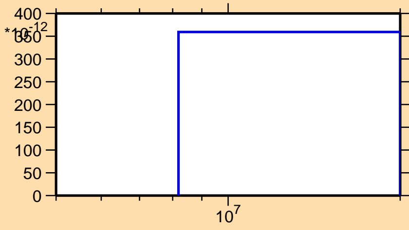
\sigma vs. E for ^{93}\text{Kr}(n,2n\alpha)
