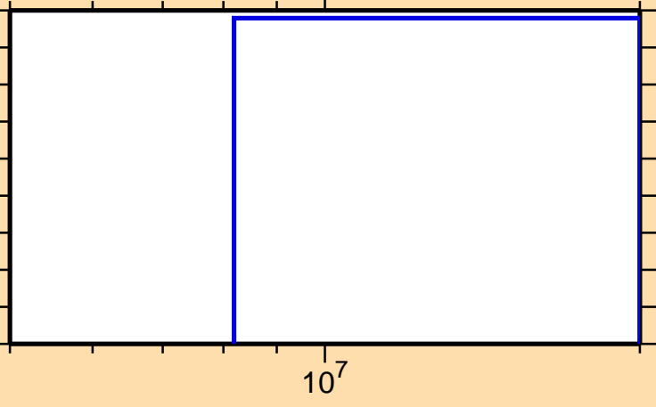
\sigma vs. E for ^{93}\text{Kr}(n,np)
