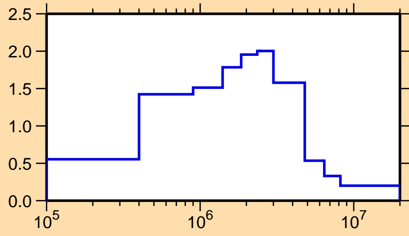
\sigma vs. E for ^{93}\text{Kr}(n,\text{inel.})
