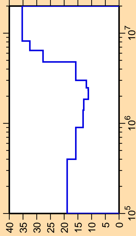
\Delta\sigma/\sigma vs. E for ^{93}\text{Kr}(n,\text{inel.})
