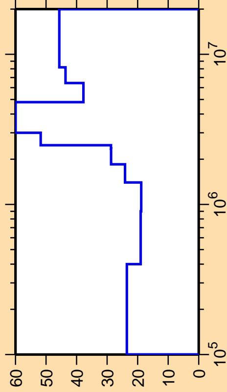
\Delta\sigma/\sigma vs. E for ^{93}\text{Kr}(n,n_2)
