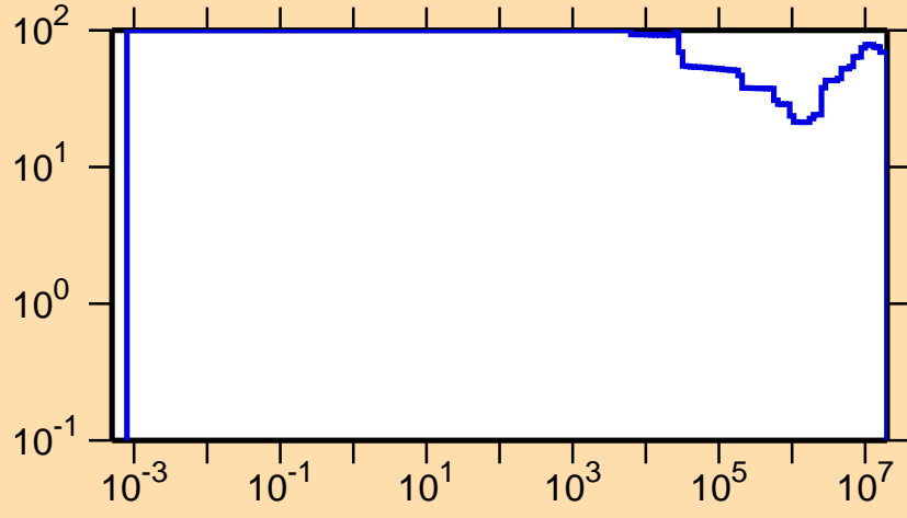
\Delta\sigma/\sigma vs. E for ^{119}\text{La}(n,p)
