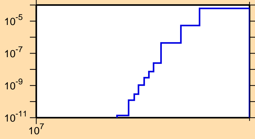
\sigma vs. E for ^{119}\text{La}(n,pt)
