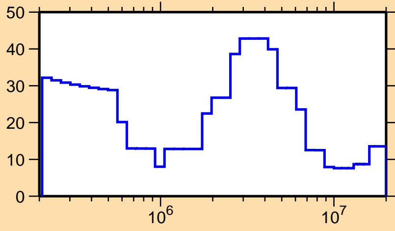
\Delta\sigma/\sigma vs. E for ^{119}\text{La}(n, el.)
