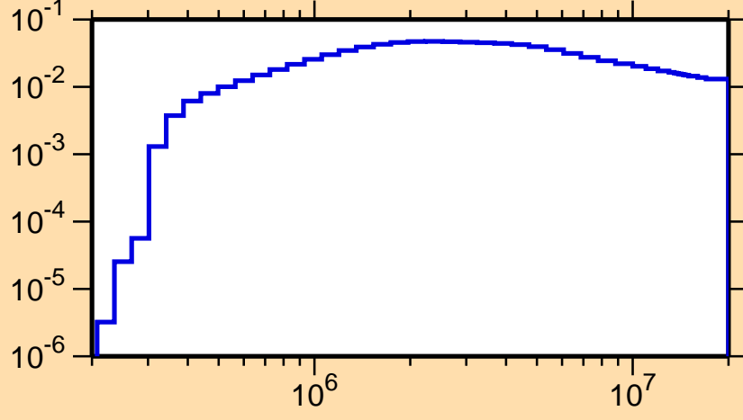
\sigma vs. E for ^{119}\text{La}(n,n_1)
