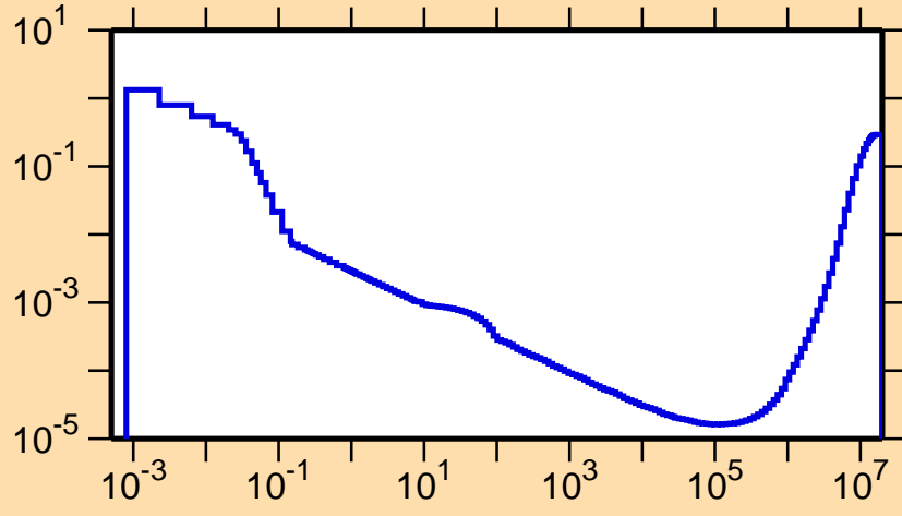
\sigma vs. E for ^{119}\text{La}(n,p\alpha)
