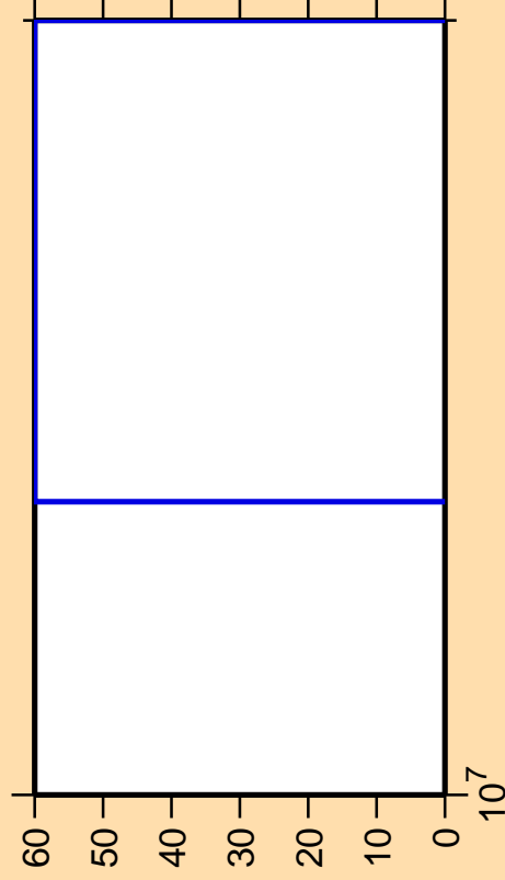
\Delta\sigma/\sigma vs. E for ^{119}\text{La}(n,pt)
