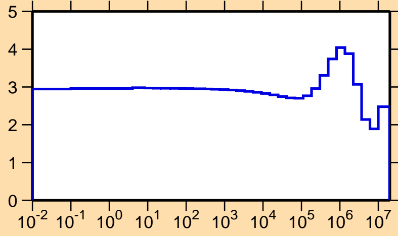
\sigma vs. E for ^{119}\text{La}(n,\text{el.})
