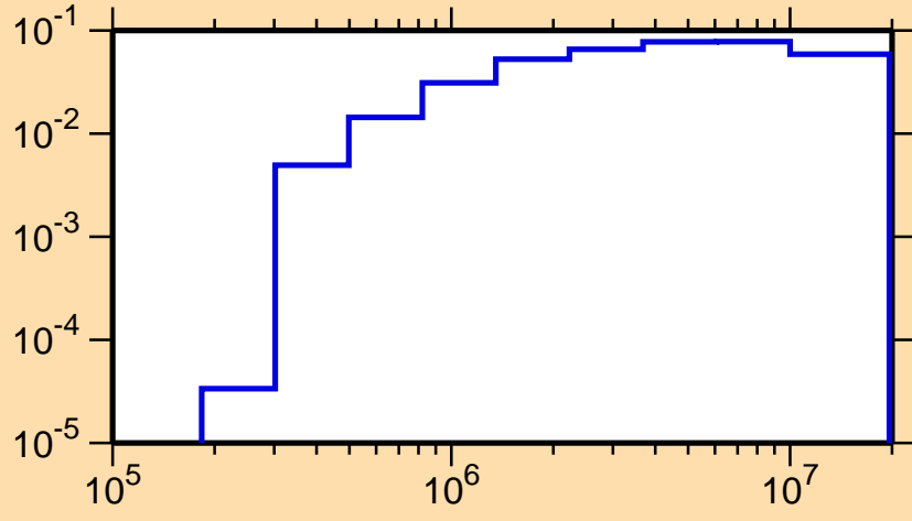
\sigma vs. E for ^{119}\text{La}(n,\text{inel.})
