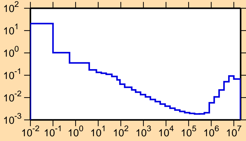
\sigma vs. E for ^{119}\text{La}(n,\alpha)
