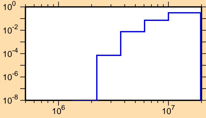
\sigma vs. E for ^{120}\text{La}(n,np)
