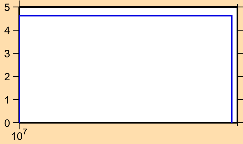
\Delta\sigma/\sigma vs. E for ^{120}\text{La}(n,\text{tot.})
