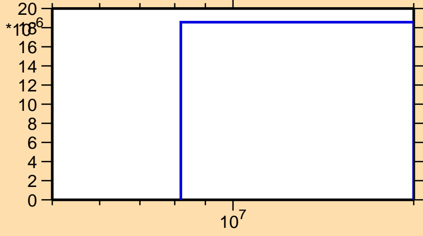
\sigma vs. E for ^{120}\text{La}(n,\text{pt})
