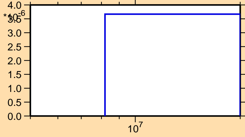
\sigma vs. E for ^{120}\text{La}(n,2np)
