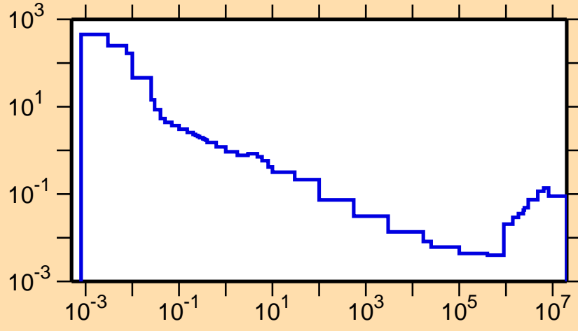
\sigma vs. E for ^{120}\text{La}(n,\alpha)
