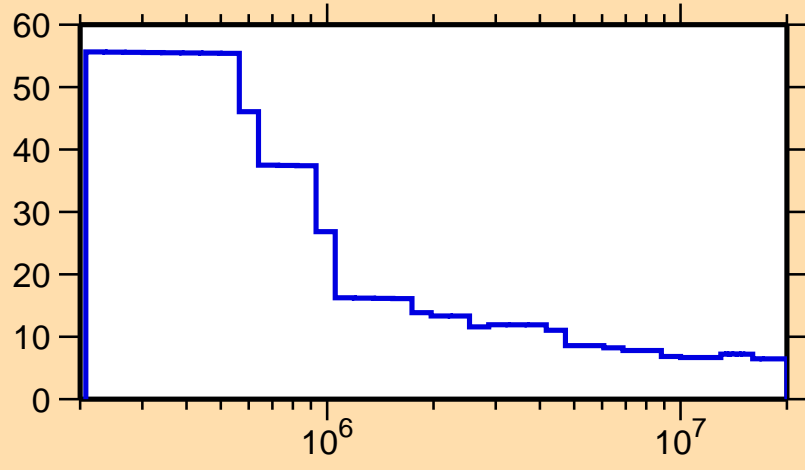
\Delta\sigma/\sigma vs. E for ^{121}\text{La}(n,\text{nonel.})
