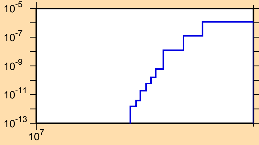
\sigma vs. E for ^{121}\text{La}(n,\text{nd})
