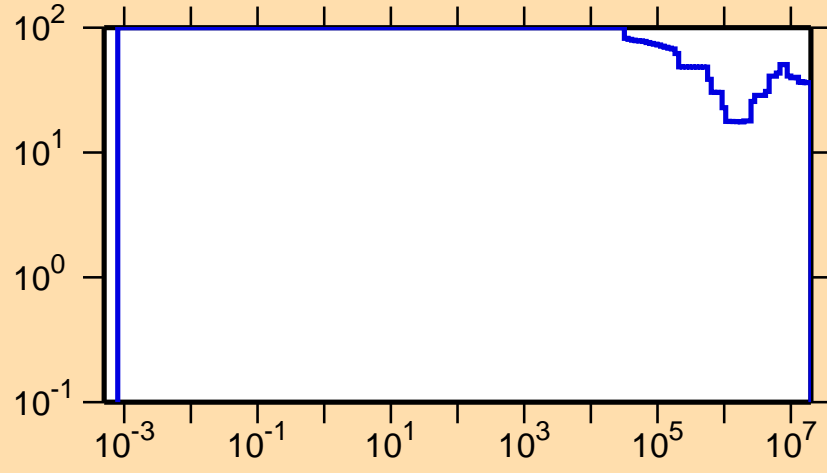
\Delta\sigma/\sigma vs. E for ^{121}\text{La}(n,p)
