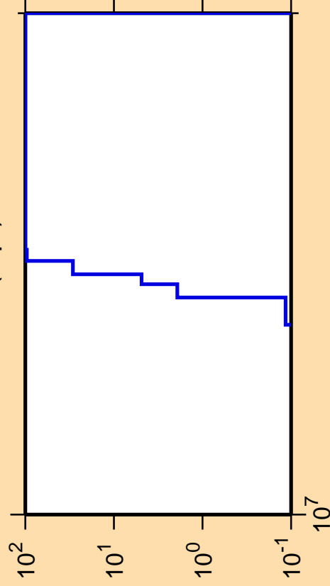
\Delta\sigma/\sigma vs. E for ^{121}\text{La}(n,pt)
