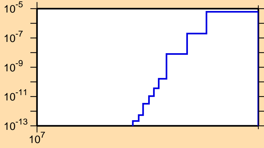
\sigma vs. E for ^{121}\text{La}(n,pt)
