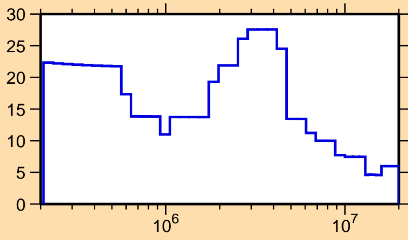
\Delta\sigma/\sigma vs. E for ^{121}\text{La}(n,\text{el.})
