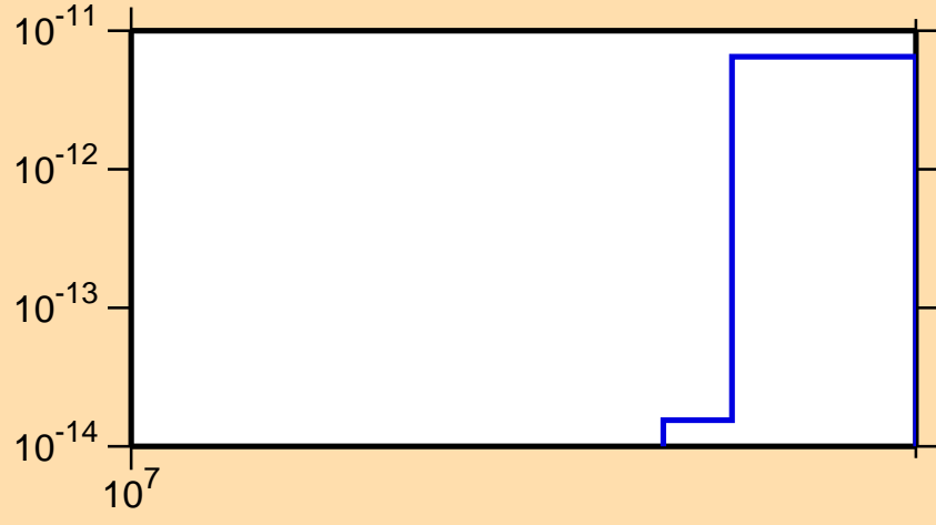
\sigma vs. E for ^{121}\text{La}(n,2n\alpha)
