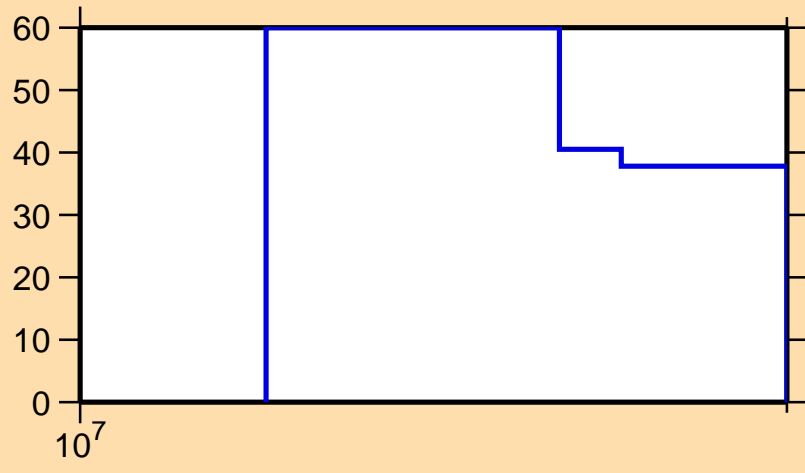
\Delta\sigma/\sigma vs. E for ^{121}\text{La}(n,2n)
