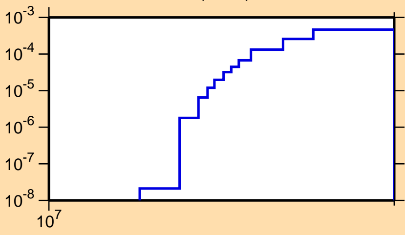
\sigma vs. E for ^{121}\text{La}(n,2n)
