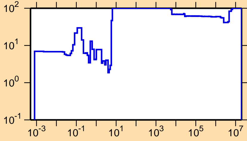
\Delta\sigma/\sigma vs. E for ^{121}\text{La}(n,\gamma)
