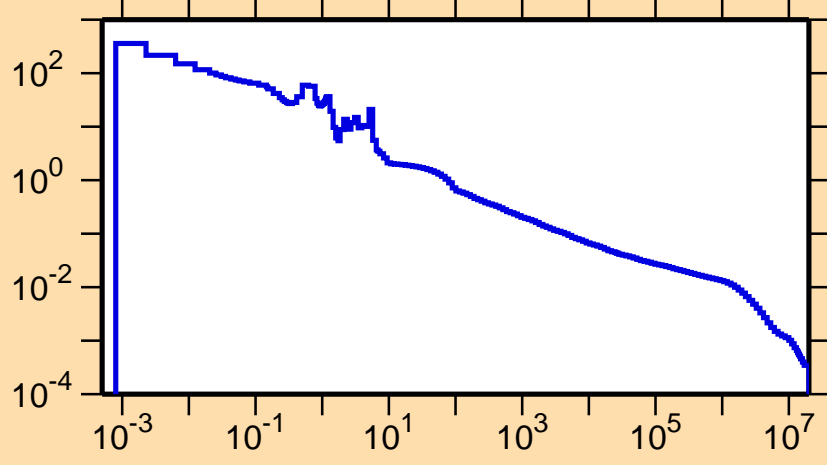
\sigma vs. E for ^{121}\text{La}(n,\gamma)
