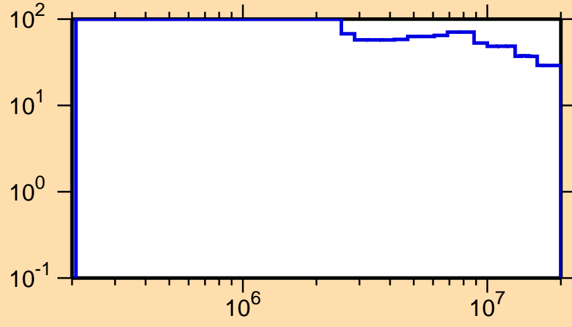
\Delta\sigma/\sigma vs. E for ^{121}\text{La}(n,n_1)
