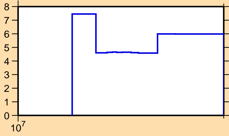
\Delta\sigma/\sigma vs. E for ^{121}\text{La}(n,\text{el.})
