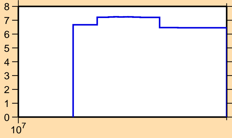
\Delta\sigma/\sigma vs. E for ^{121}\text{La}(n,\text{nonel.})
