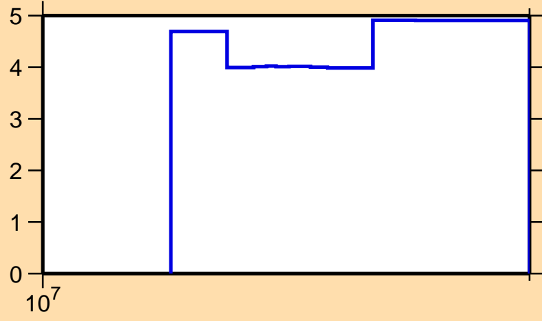
\Delta\sigma/\sigma vs. E for ^{121}\text{La}(n,\text{tot.})
