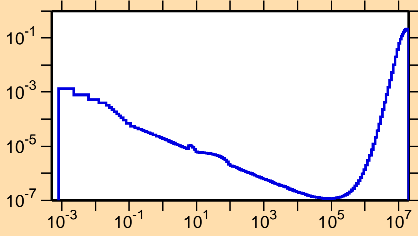
\sigma vs. E for ^{121}\text{La}(n,p\alpha)
