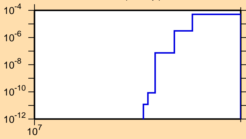
\sigma vs. E for ^{121}\text{La}(n,2np)
