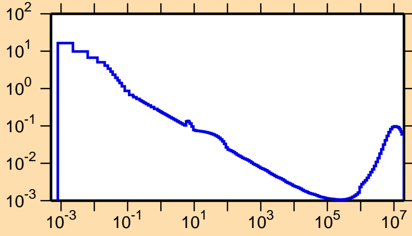
\sigma vs. E for ^{121}\text{La}(n,\alpha)
