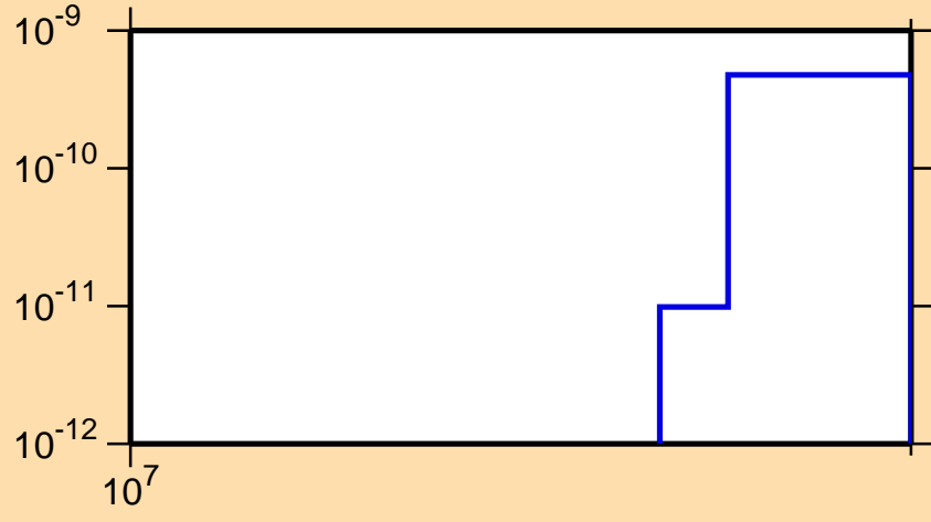
\sigma vs. E for ^{121}\text{La} (mt 34)
