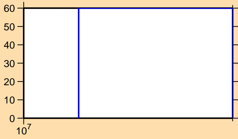
\Delta\sigma/\sigma vs. E for ^{121}\text{La}(n,\text{inel.})
