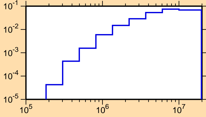
\sigma vs. E for ^{121}\text{La}(n,n\text{cont.})
