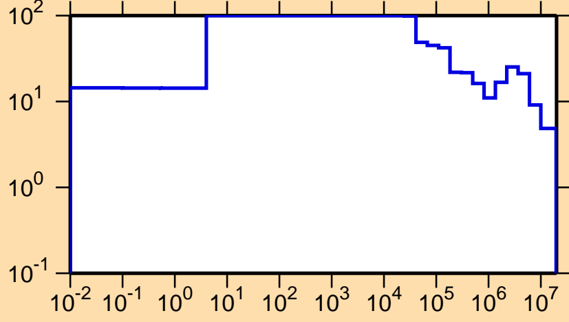
\Delta\sigma/\sigma vs. E for ^{121}\text{La}(n,el.)
