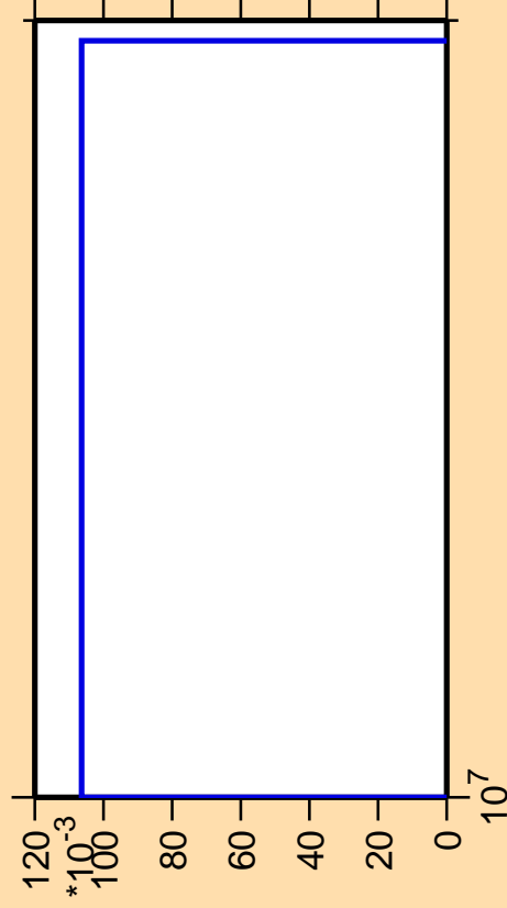
\Delta\sigma/\sigma vs. E for ^{121}\text{La}(n,nt)
