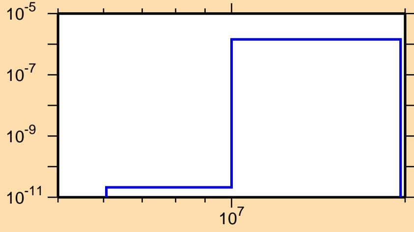
\sigma vs. E for ^{121}\text{La}(\text{mt117})
