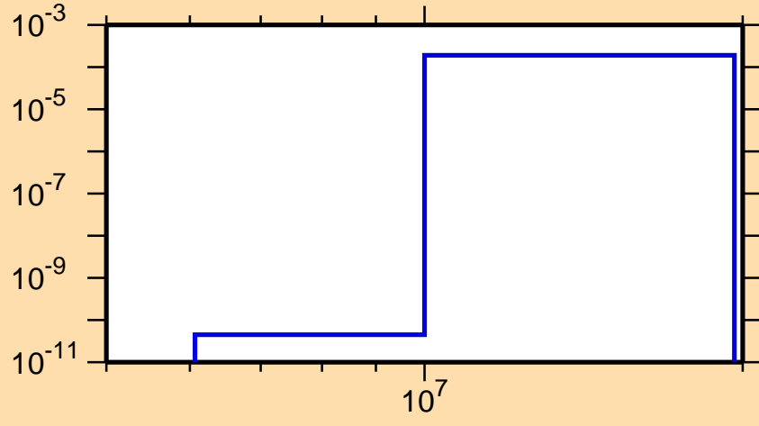
\sigma vs. E for ^{122}\text{La}(n,pd)
