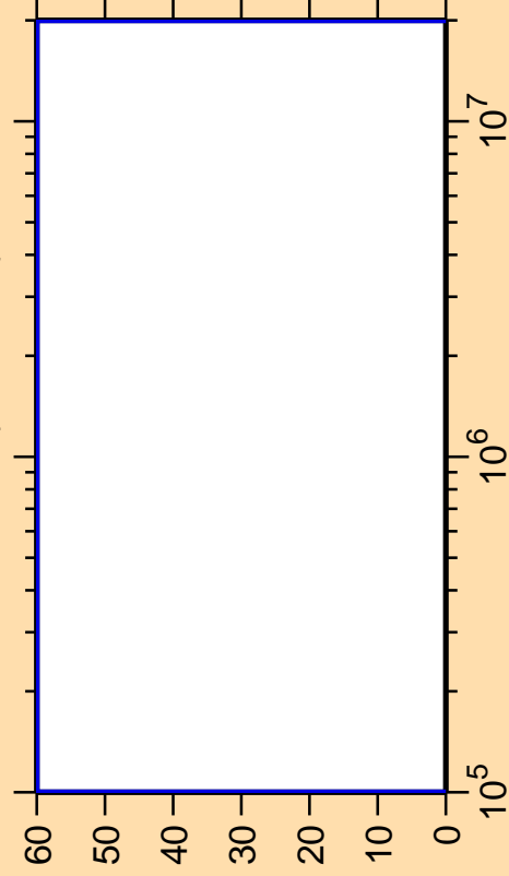
\Delta\sigma/\sigma vs. E for ^{122}\text{La}(n,\text{ncont.})
