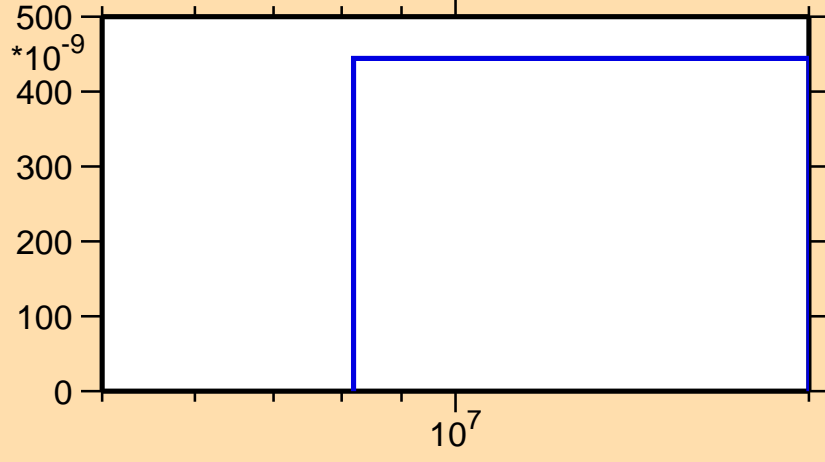
\sigma vs. E for ^{122}\text{La}(\text{mt117})
