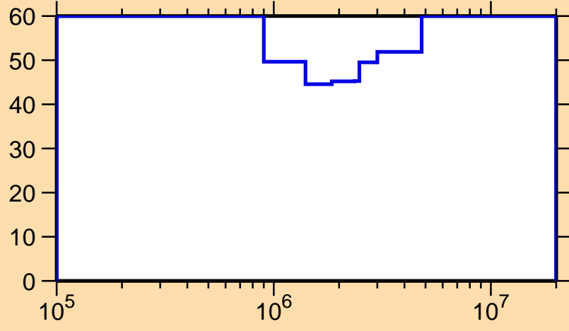
\Delta\sigma/\sigma vs. E for ^{123}\text{La}(n,n_1)
