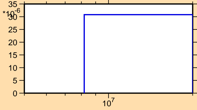
\sigma vs. E for ^{123}\text{La}(n,pd)
