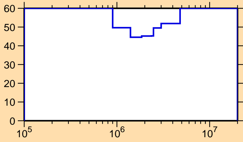
\Delta\sigma/\sigma vs. E for ^{123}\text{La}(n,n_1)
