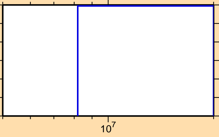
\sigma vs. E for ^{123}\text{La}(\text{mt117})
