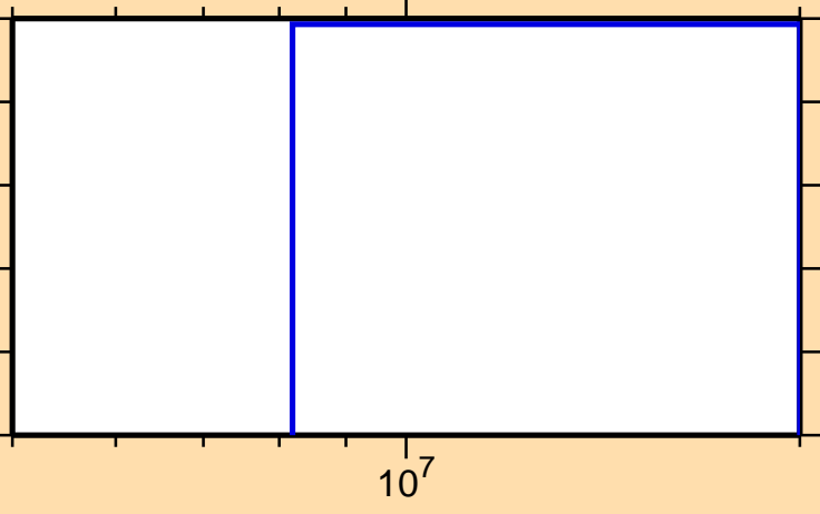
\sigma vs. E for ^{123}\text{La}(n,\text{nd})
