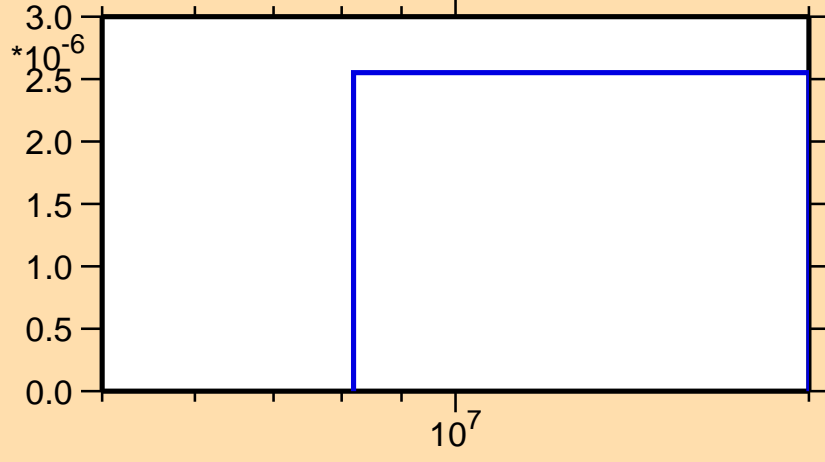
\sigma vs. E for ^{123}\text{La}(n,2np)
