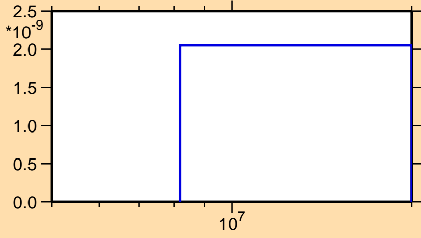
\sigma vs. E for ^{123}\text{La}(n,\text{pt})
