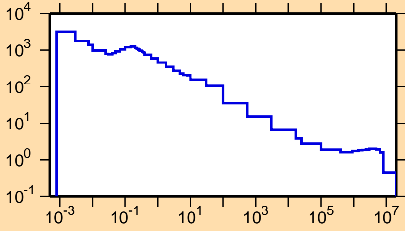
\sigma vs. E for ^{123}\text{La}(n,p)
