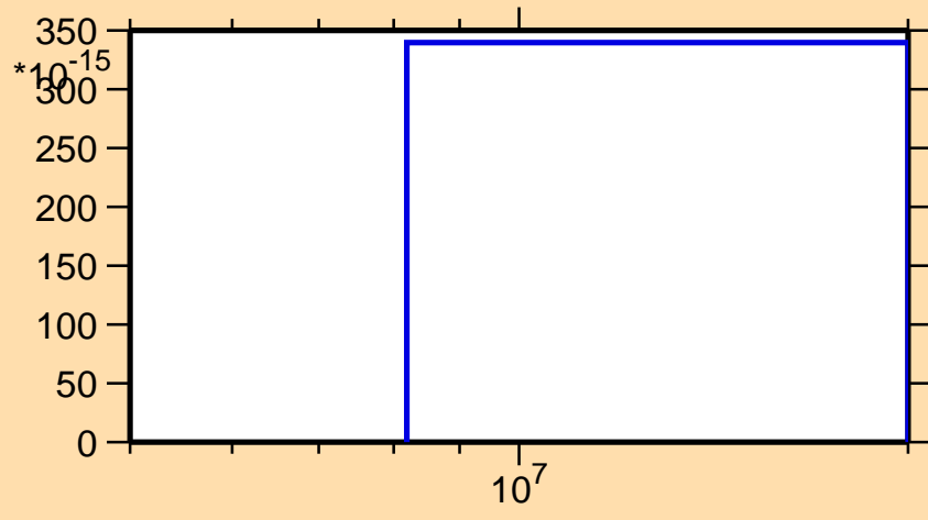
\sigma vs. E for ^{123}\text{La}(n,nt)
