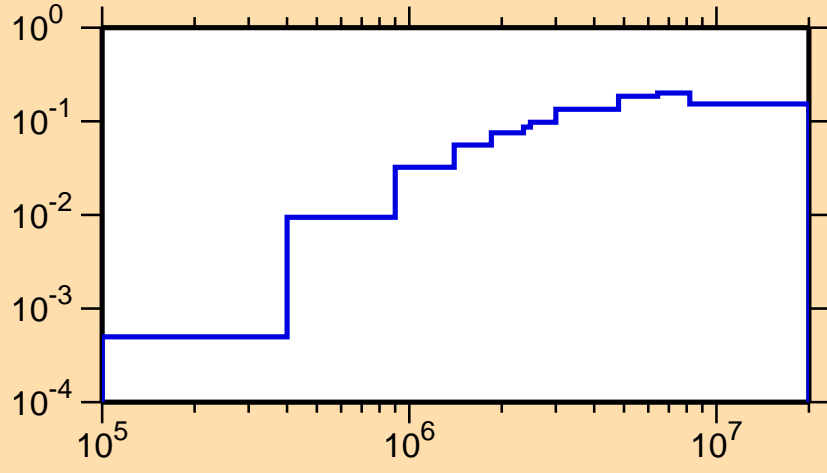
\sigma vs. E for ^{123}\text{La}(n,n\text{cont.})
