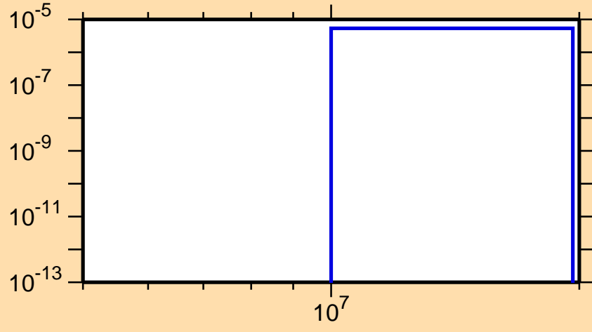
\sigma vs. E for ^{124}\text{La}(n,nd)
