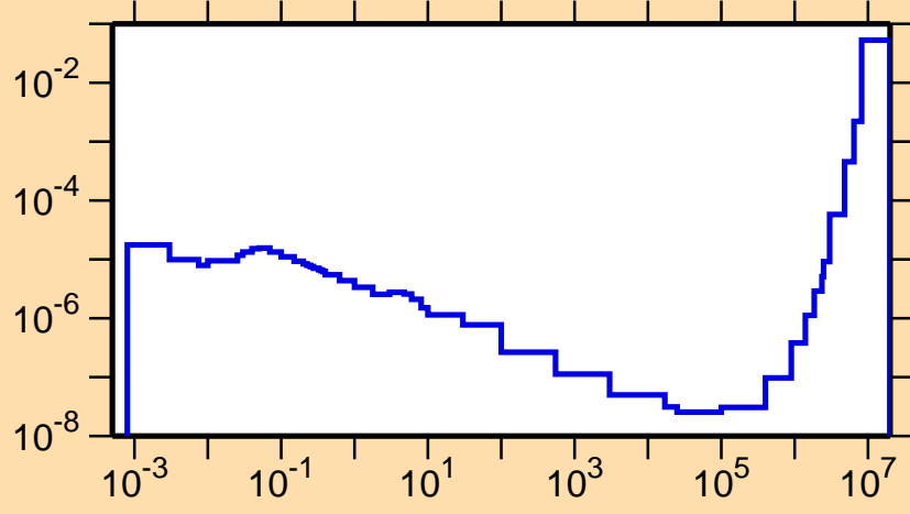
\sigma vs. E for ^{124}\text{La}(n,p\alpha)
