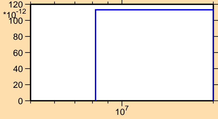
\sigma vs. E for ^{124}\text{La} (mt 34)
