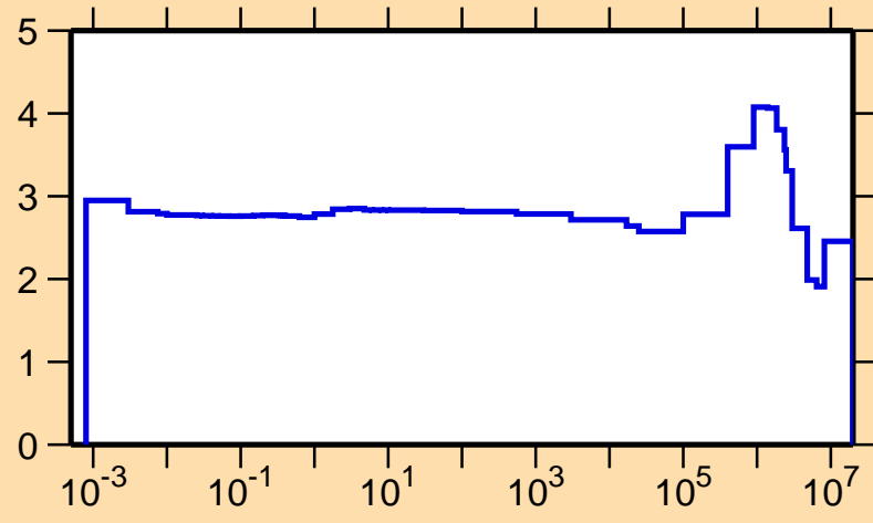
\sigma vs. E for ^{124}\text{La}(n,\text{el.})
