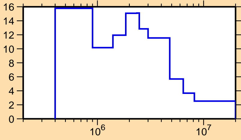
\Delta\sigma/\sigma vs. E for ^{124}\text{La}(n,\text{tot.})
