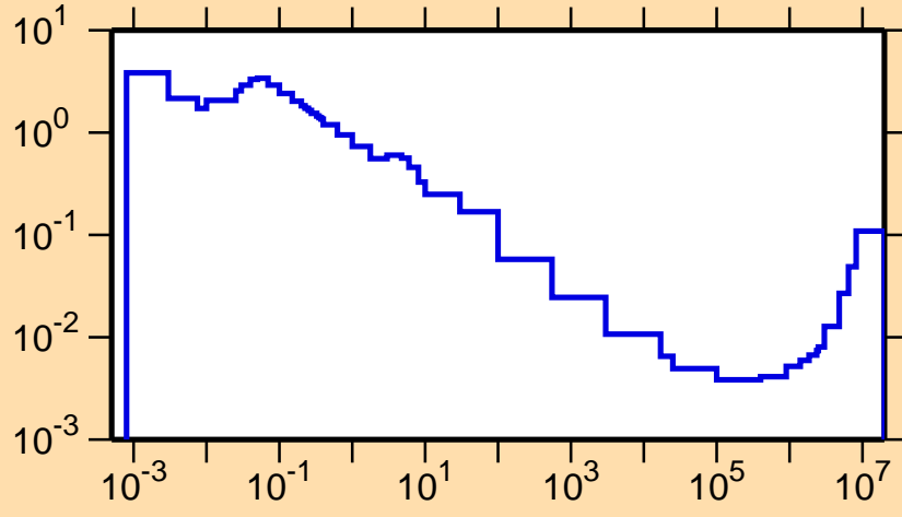
\sigma vs. E for ^{124}\text{La}(n,\alpha)
