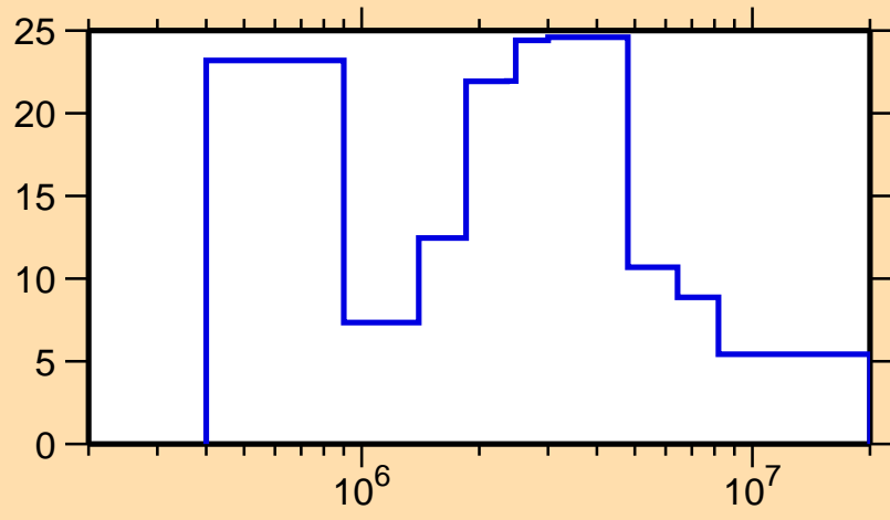
\Delta\sigma/\sigma vs. E for ^{124}\text{La}(n,\text{el.})
