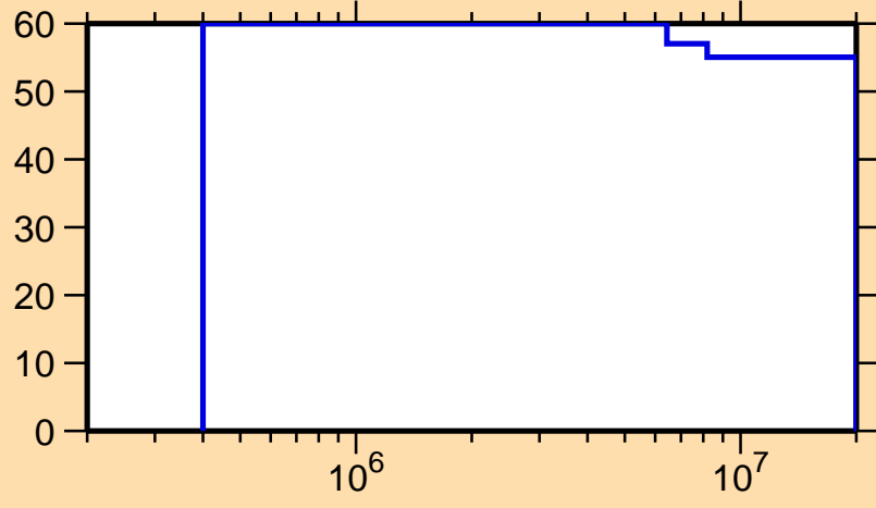
\Delta\sigma/\sigma vs. E for ^{124}\text{La}(n,n_1)
