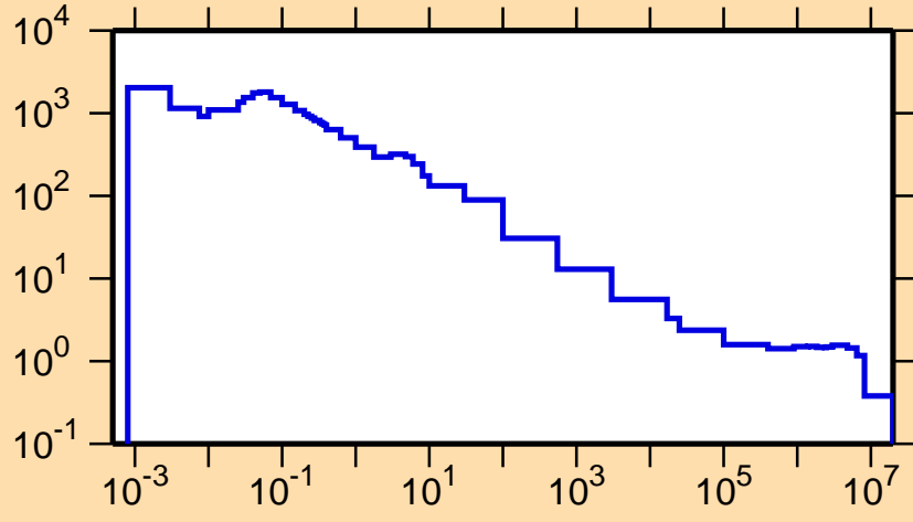
\sigma vs. E for ^{124}\text{La}(n,p)
