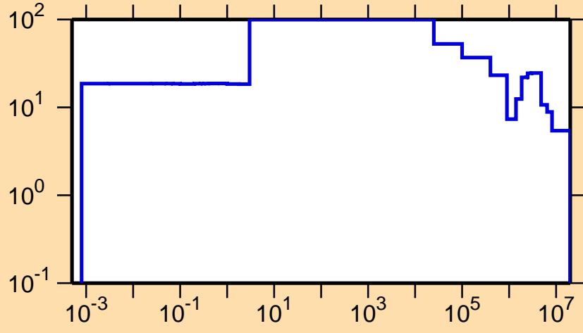
\Delta\sigma/\sigma vs. E for ^{124}\text{La}(n,\text{el.})
