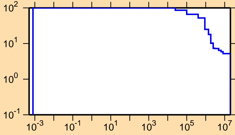
\Delta\sigma/\sigma vs. E for ^{124}\text{La}(n,\text{nonel.})
