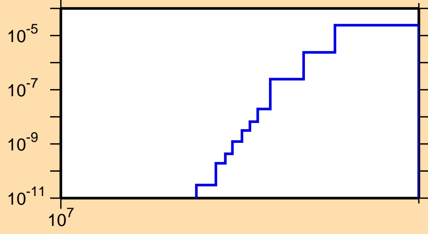
\sigma vs. E for ^{124}\text{La}(n,pt)
