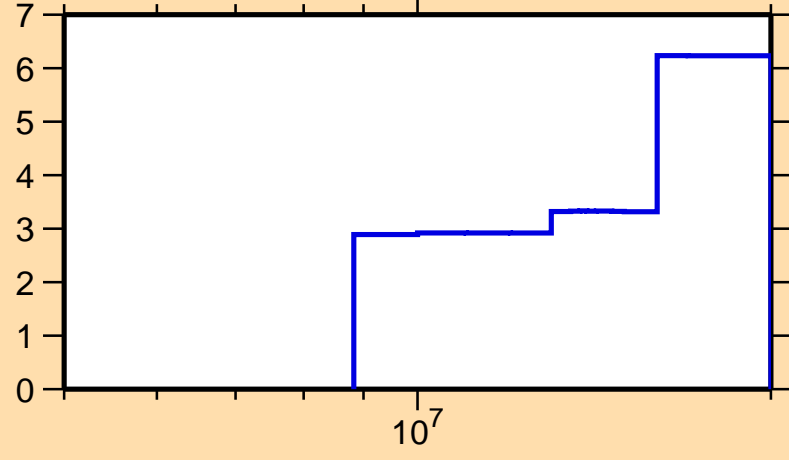
\Delta\sigma/\sigma vs. E for ^{124}\text{La}(n,\text{tot.})
