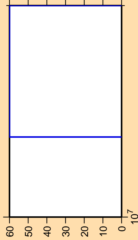
\Delta\sigma/\sigma vs. E for ^{124}\text{La}(n,pt)
