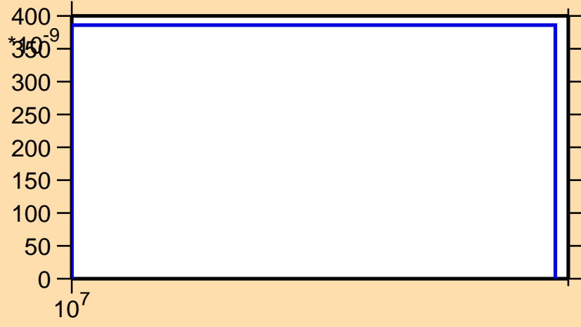
\sigma vs. E for ^{124}\text{La}(n,\text{pt})
