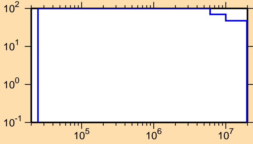
\Delta\sigma/\sigma vs. E for ^{124}\text{La}(n,n\text{cont.})
