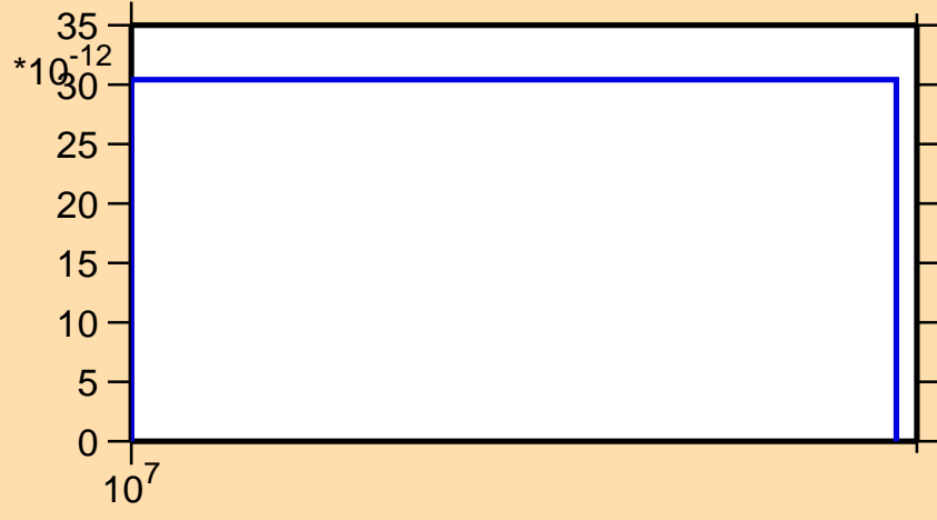
\sigma vs. E for ^{124}\text{La}(n,nt)
