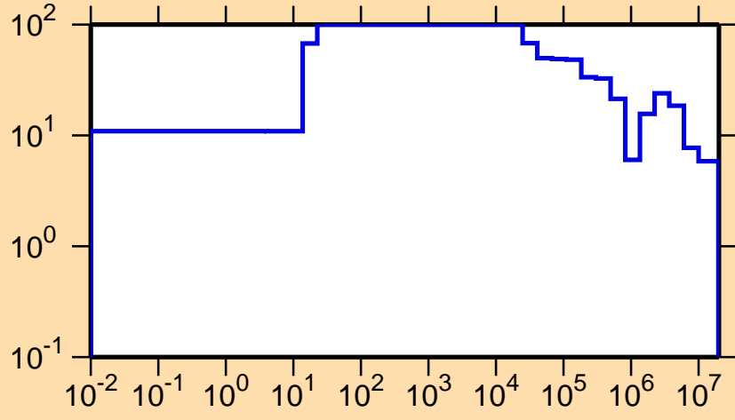
\Delta\sigma/\sigma vs. E for ^{124}\text{La}(n,el.)
