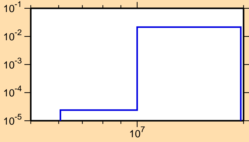
\sigma vs. E for ^{124}\text{La}(n,2n)
