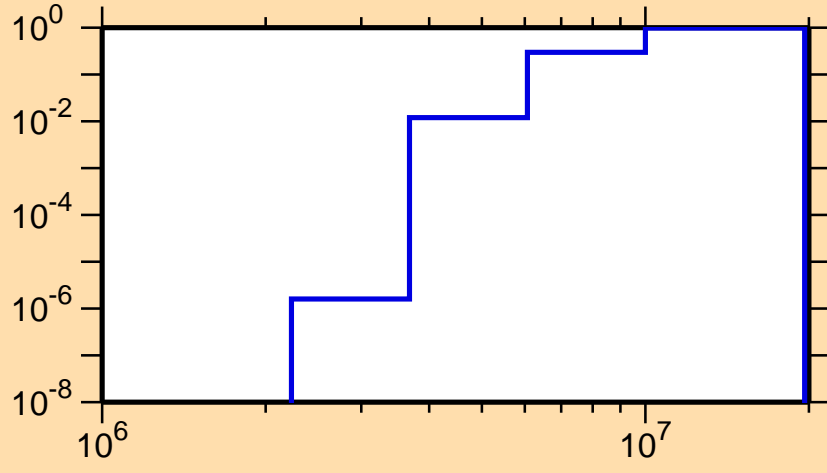
\sigma vs. E for ^{124}\text{La}(n,np)
