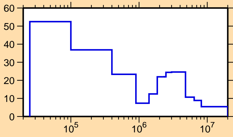
\Delta\sigma/\sigma vs. E for ^{124}\text{La}(n, el.)
