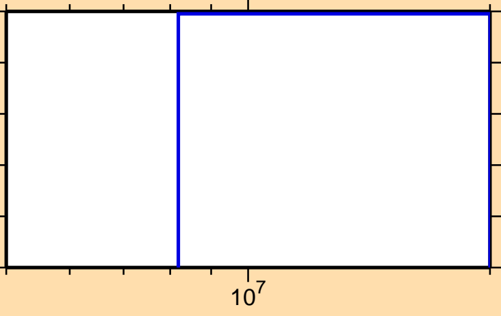
\sigma vs. E for ^{124}\text{La}(n,2np)
