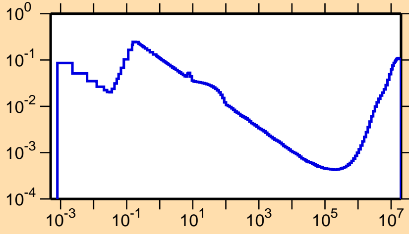
\sigma vs. E for ^{125}\text{La}(n,\alpha)
