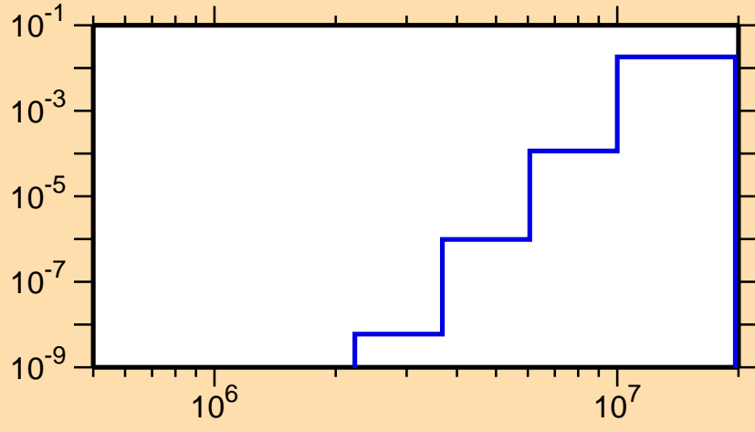
\sigma vs. E for ^{125}\text{La}(n,p\alpha)
