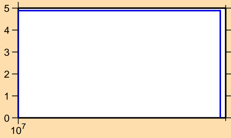
\Delta\sigma/\sigma vs. E for ^{125}\text{La}(n,\text{nonel.})
