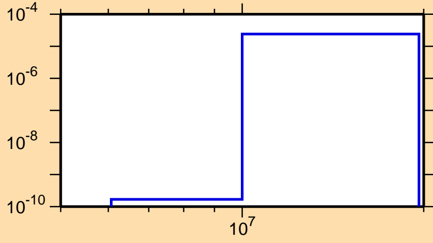
\sigma vs. E for ^{125}\text{La}(n,\text{He3})
