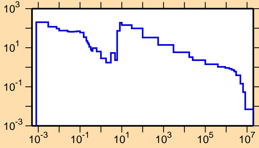
\sigma vs. E for ^{125}\text{La}(n,\gamma)
