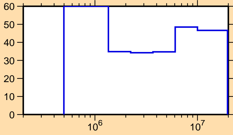
\Delta\sigma/\sigma vs. E for ^{126}\text{La}(n,n_1)
