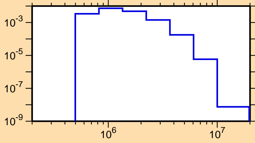
\sigma vs. E for ^{126}\text{La}(n,n_3)
