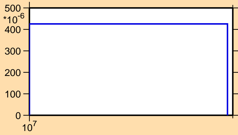
\sigma vs. E for ^{126}\text{La}(n,2np)
