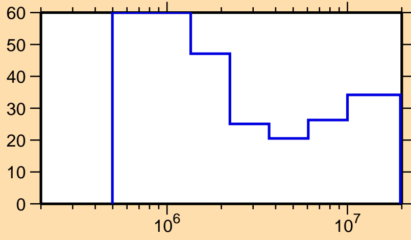
\Delta\sigma/\sigma vs. E for ^{126}\text{La}(n,n\text{cont.})
