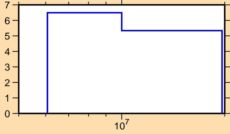
\Delta\sigma/\sigma vs. E for ^{126}\text{La}(n,\text{el.})
