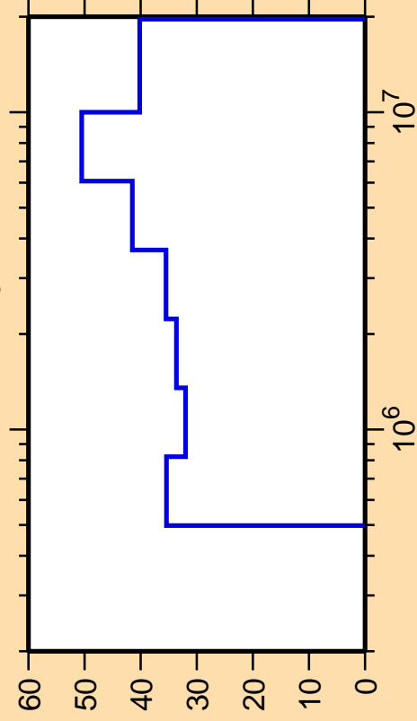
\Delta\sigma/\sigma vs. E for ^{126}\text{La}(n,n_3)
