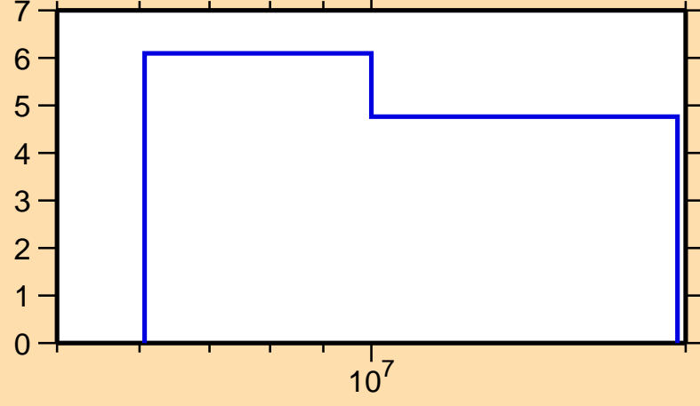
\Delta\sigma/\sigma vs. E for ^{126}\text{La}(n,\text{tot.})
