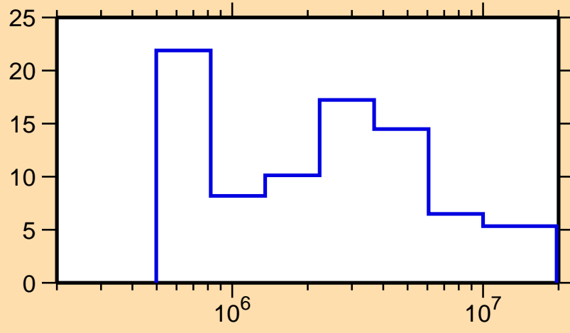
\Delta\sigma/\sigma vs. E for ^{126}\text{La}(n,\text{el.})
