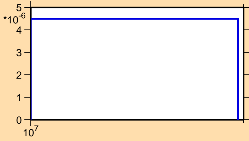
\sigma vs. E for ^{126}\text{La}(n,\text{nd})
