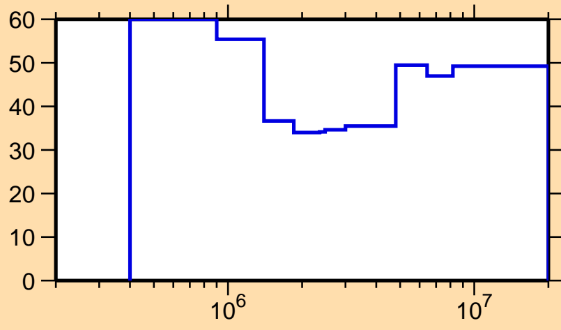
\Delta\sigma/\sigma vs. E for ^{126}\text{La}(n,n_1)
