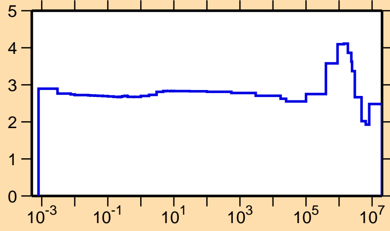
\sigma vs. E for ^{126}\text{La}(n,\text{el.})
