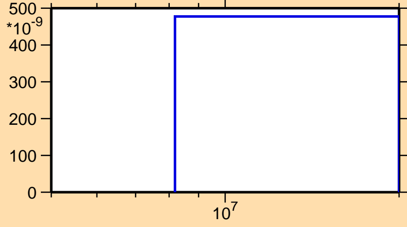
\sigma vs. E for ^{126}\text{La}(n,\text{pd})
