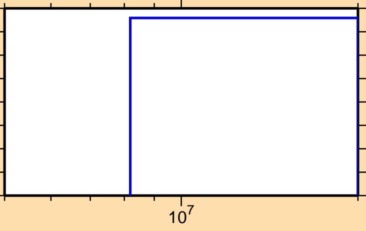
\sigma vs. E for ^{126}\text{La}(n,\text{pt})
