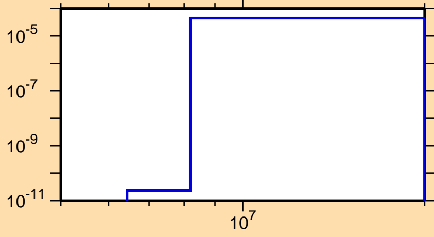
\sigma vs. E for ^{126}\text{La}(n,\text{He3})
